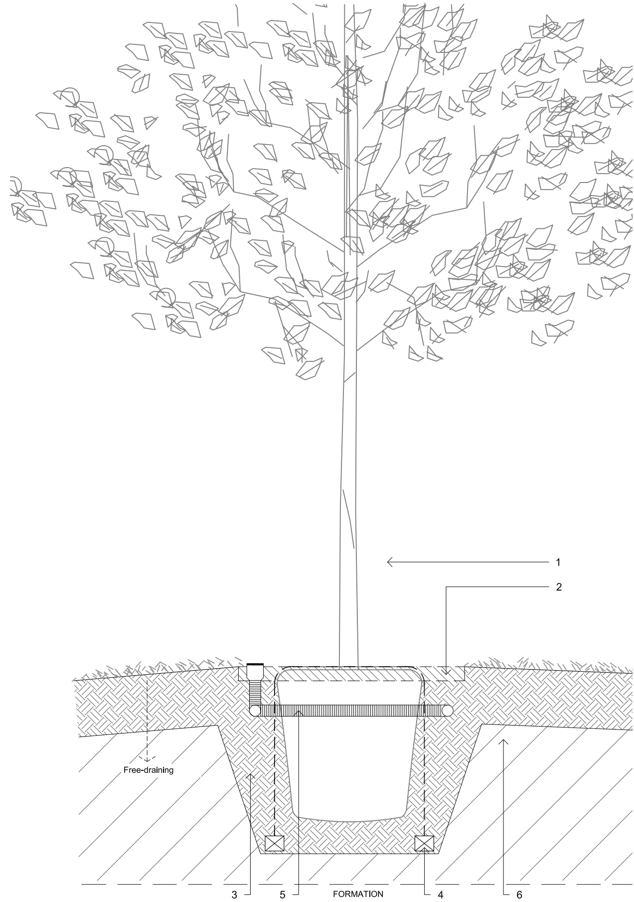
A Tree in planting 1:20 @ A3
