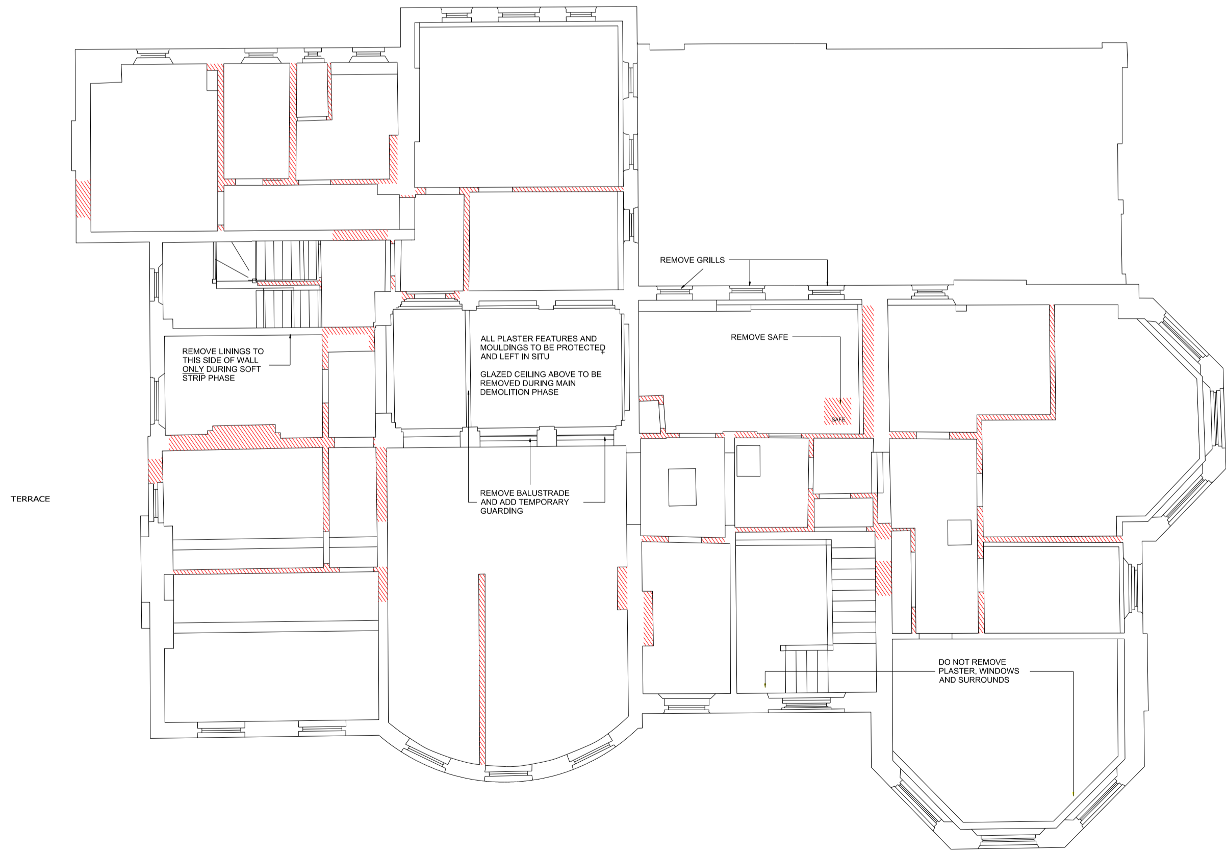
FIRST FLOOR
