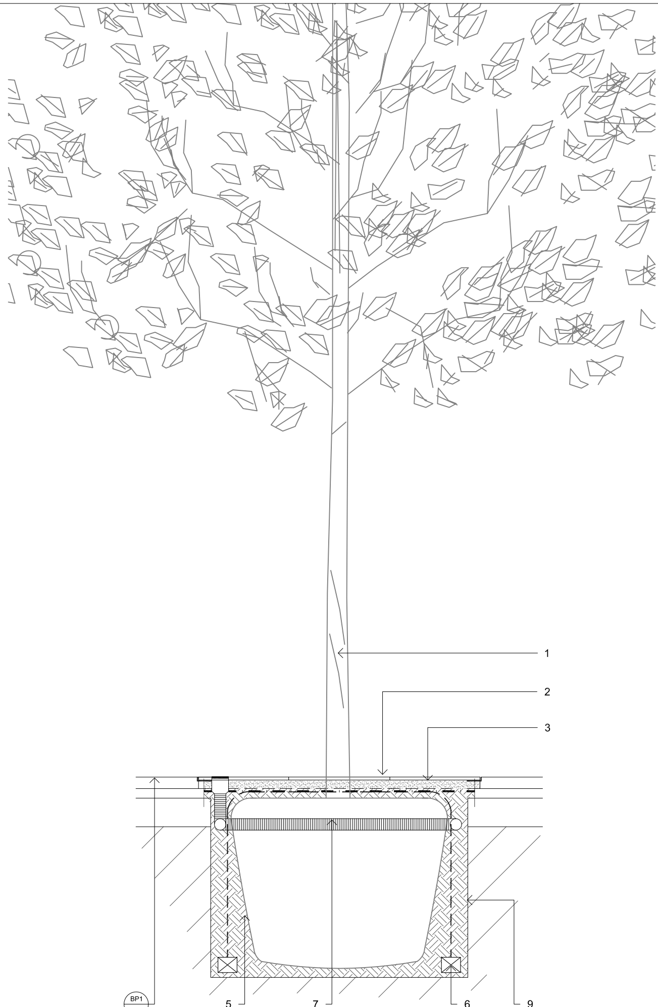
B Tree in hard paving 1:20 @ A3
