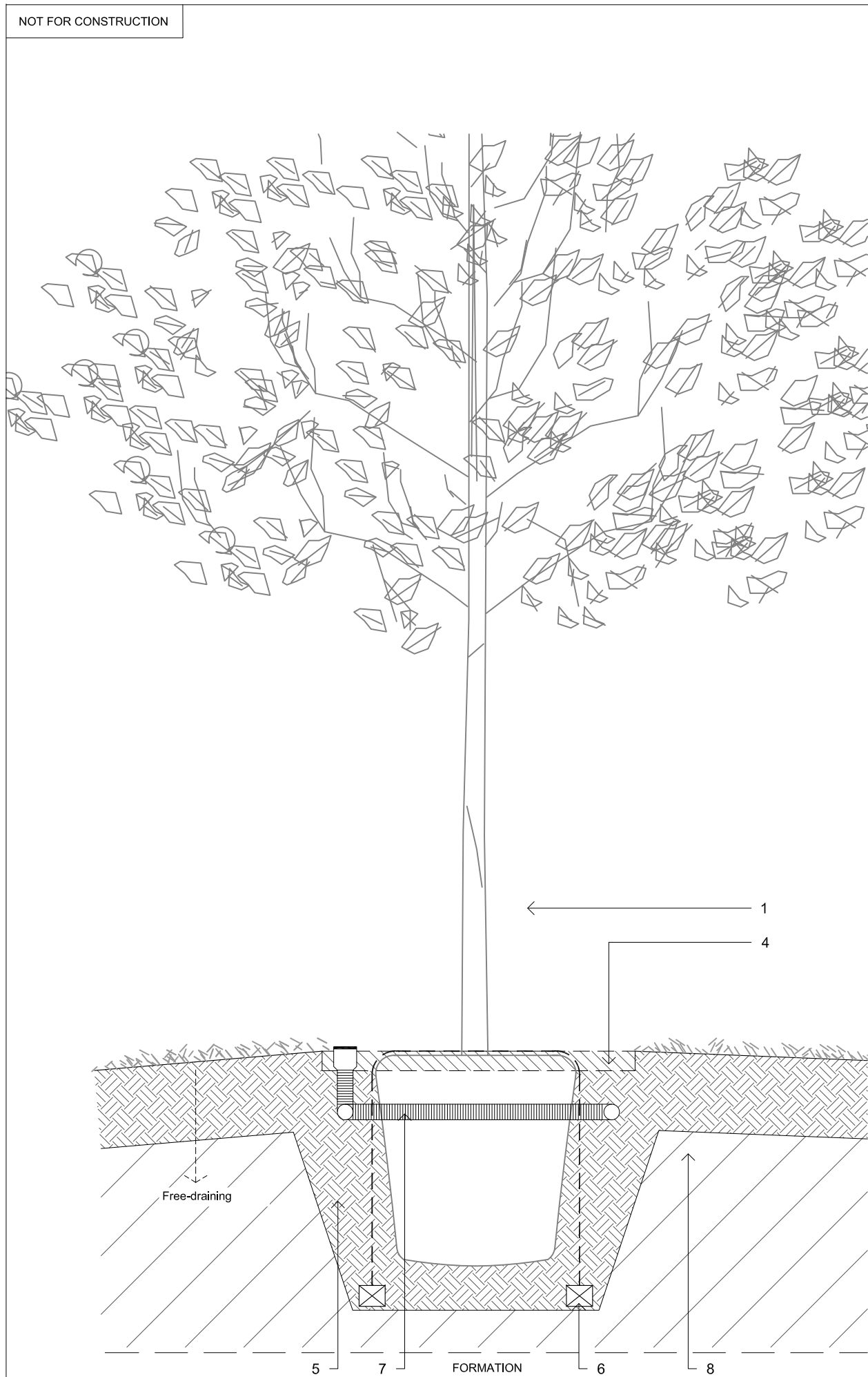
A Tree in planting 1:20 @ A3
