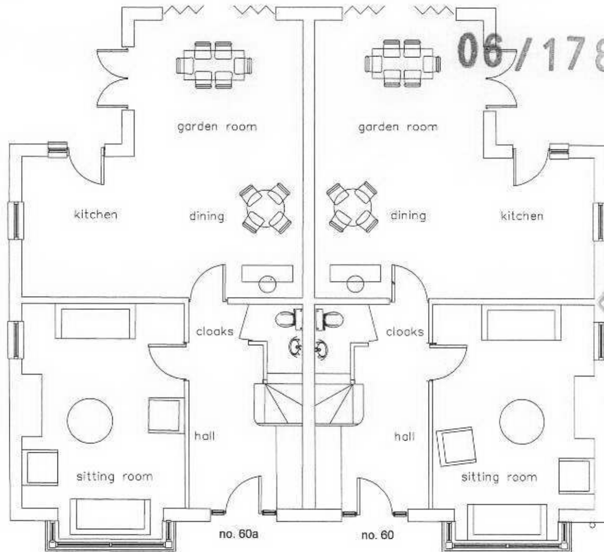
PROPOSED GROUND FLOOR 60 Derby Road East Sheen Scale 1:100
