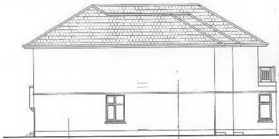
SIDE ELEVATION 4 - 4
