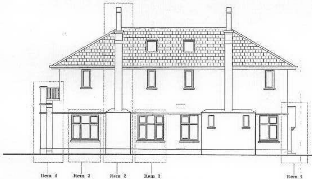
PROPOSED SIDE ELEVATION 7 - 7
