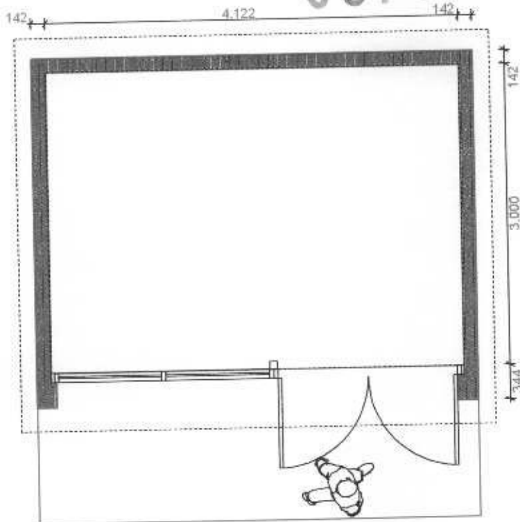
Floor Plan 1:50
