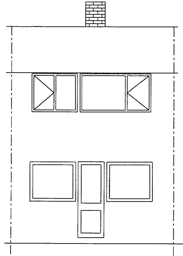
REAR ELEVATION TO GARDEN
