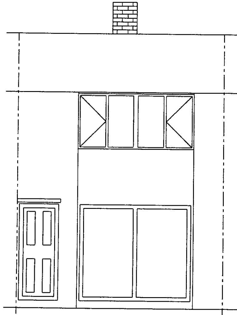
FRONT ELEVATION TO CAMBRIDGE ROAD
