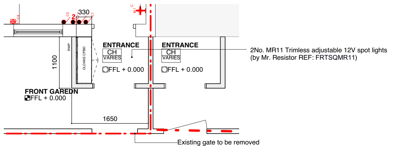
3 PR KEY PLAN 1:50
