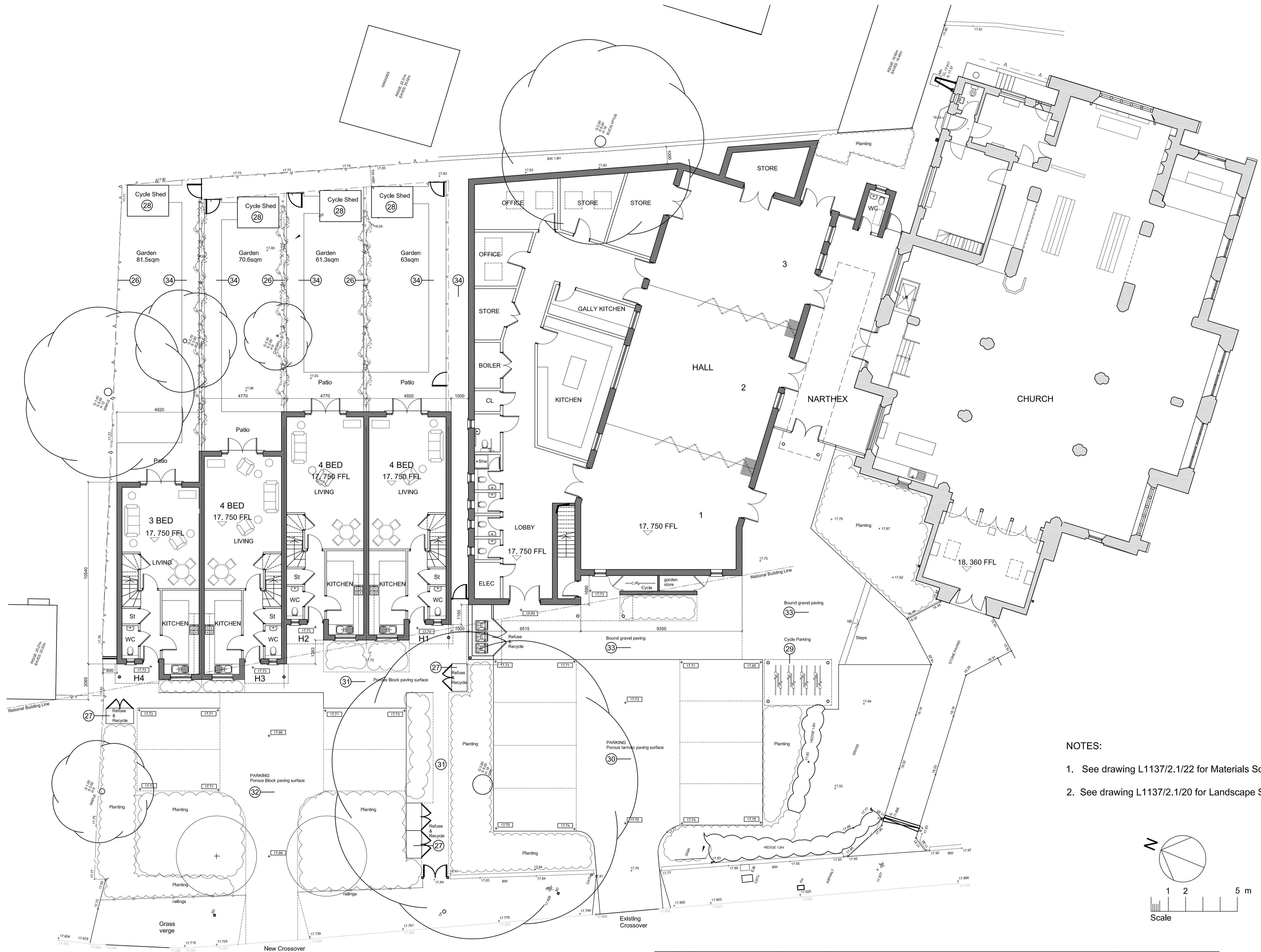
SITE & GROUND FLOOR PLAN
