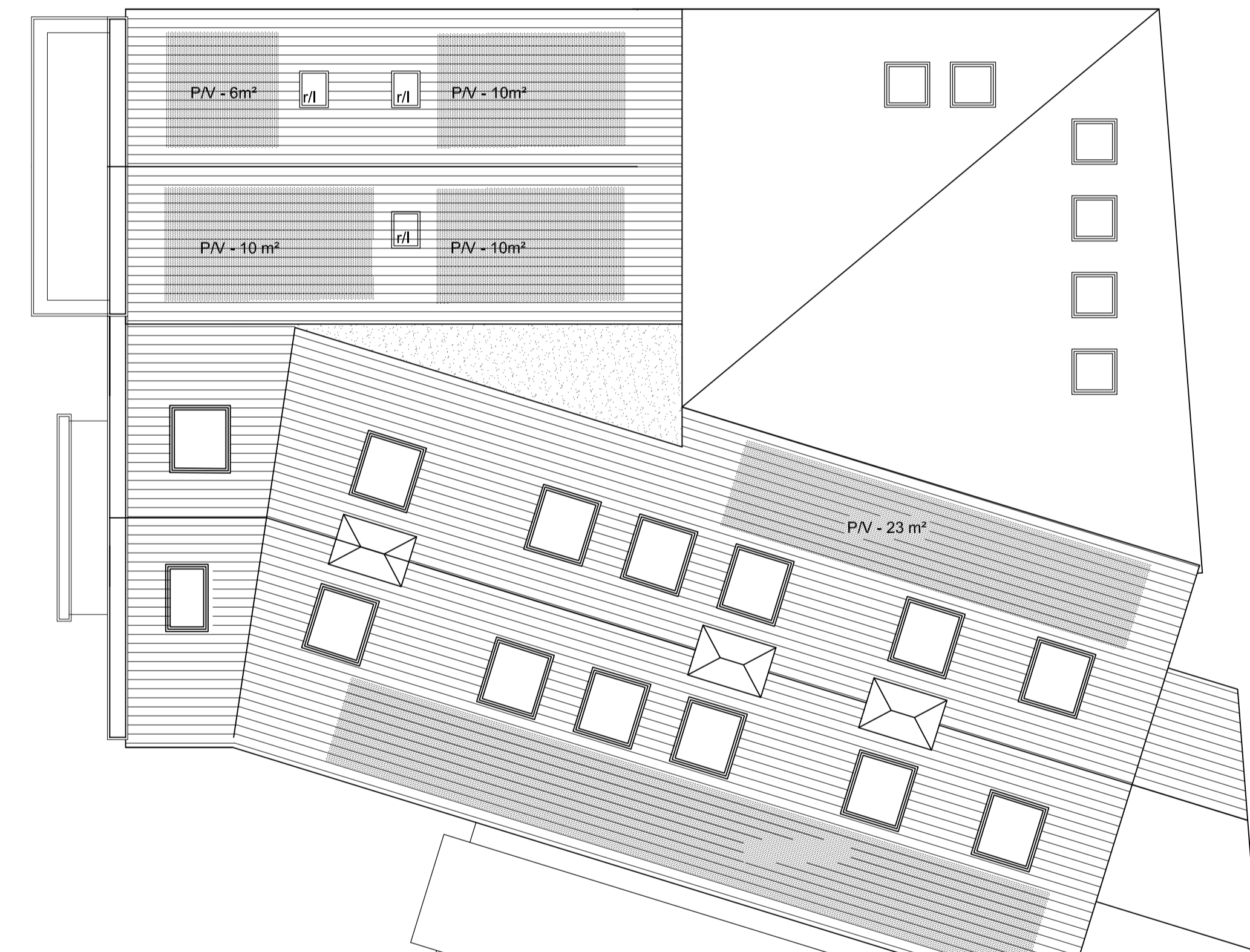
ROOF PLAN
