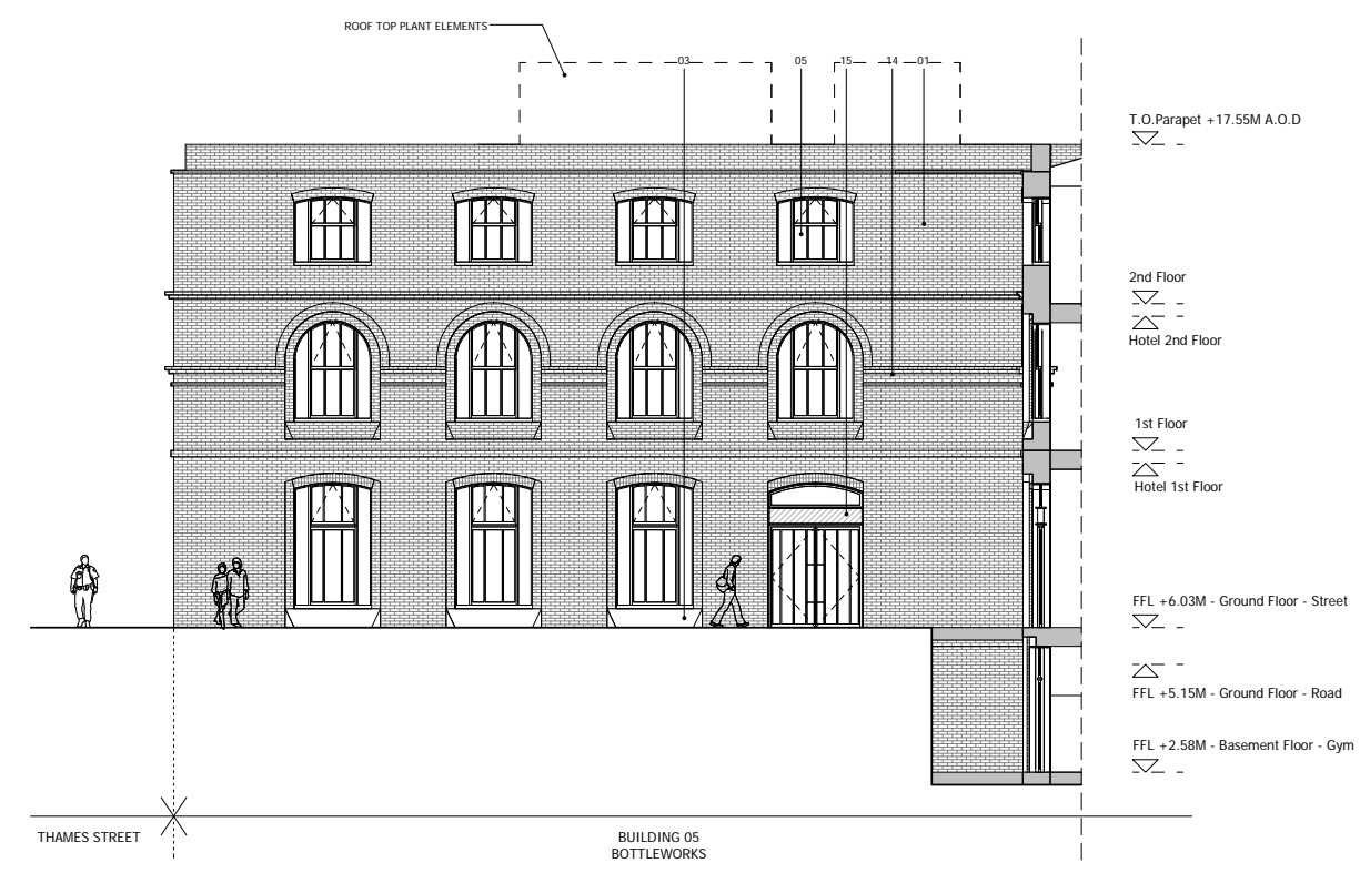
2 PROPOSED WEST ELEVATION 1 1 : 100
