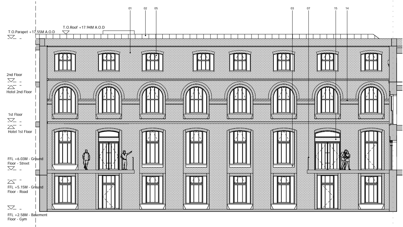
3 PROPOSED NORTH 3 1 : 100
