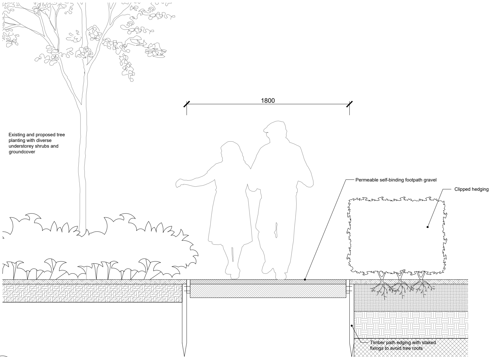
1 Footpath gravel - Detail 33 1:25 @ A4
