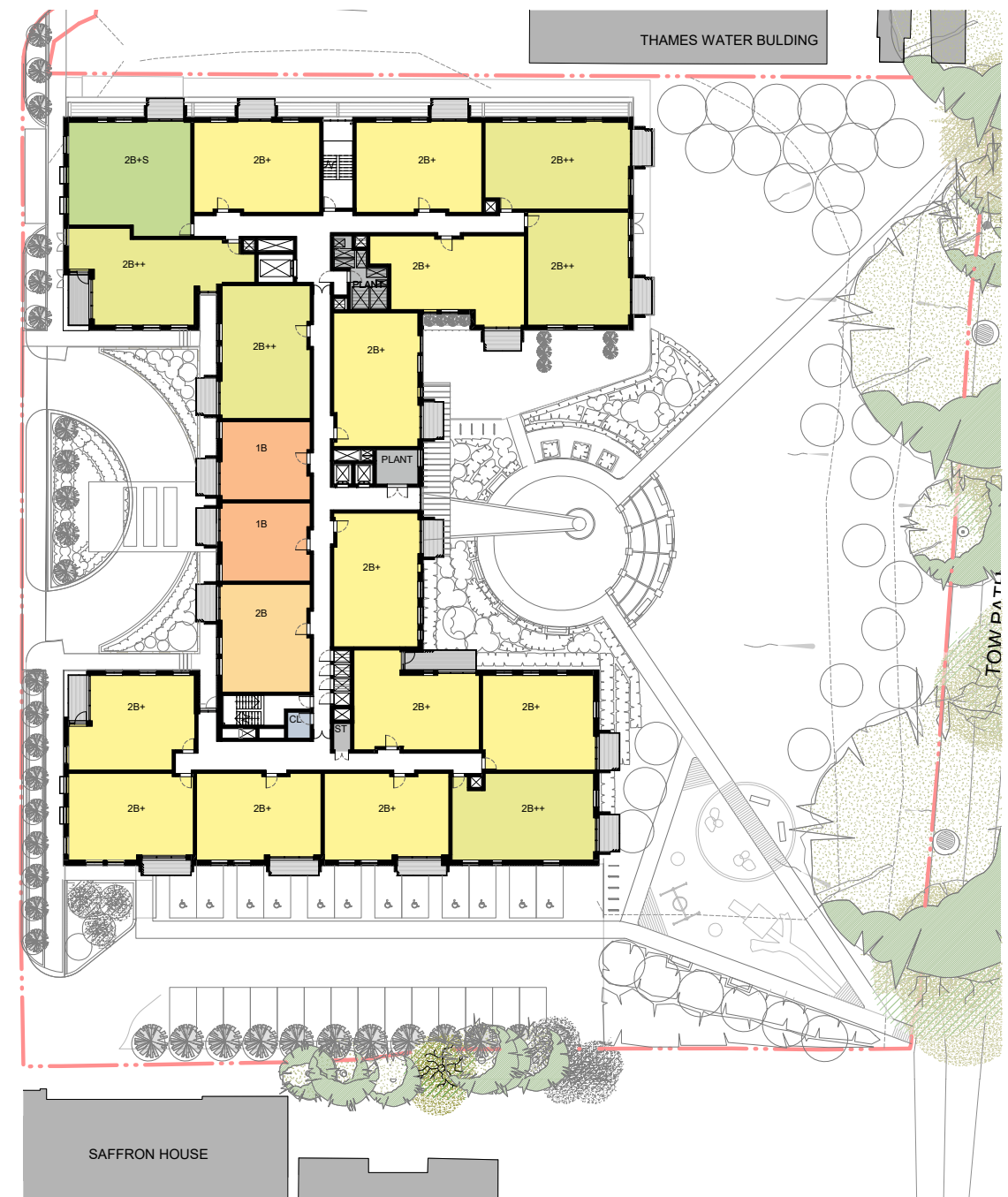
Proposed Level 3 General Arrangement
