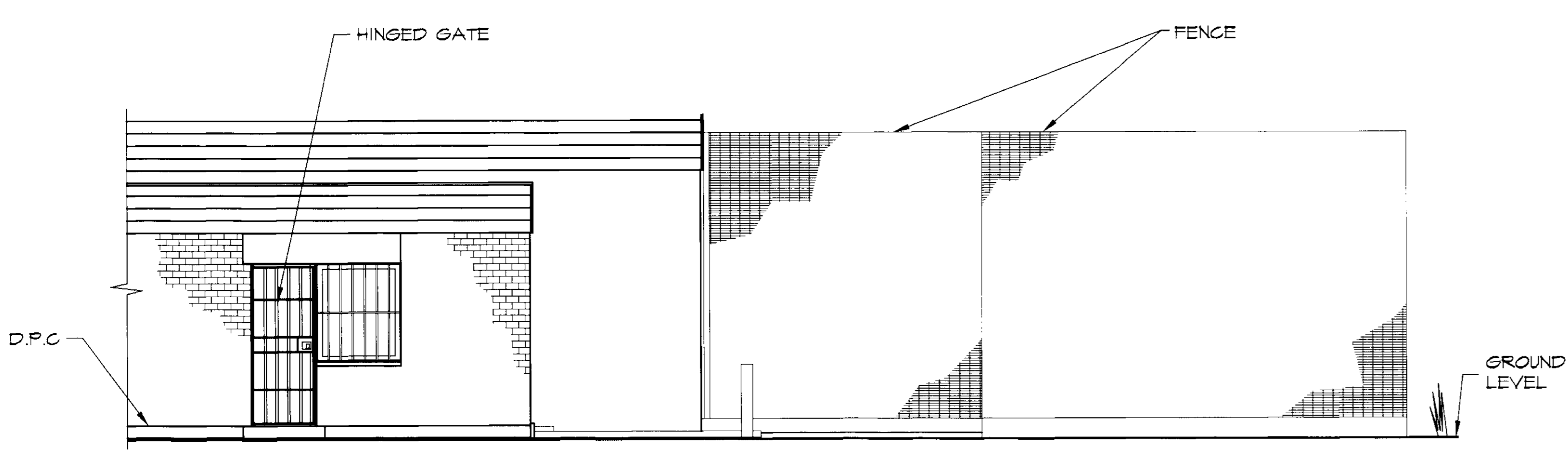
ELEVATION ON ARROW 'A'
