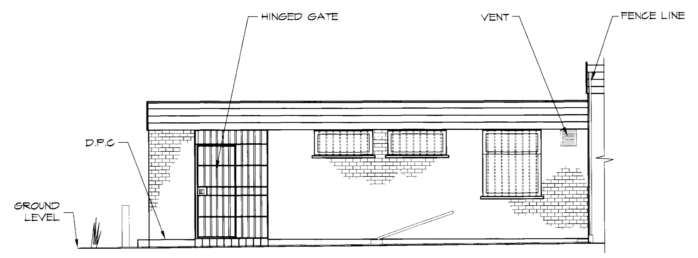
ELEVATION ON ARROW 'B'
