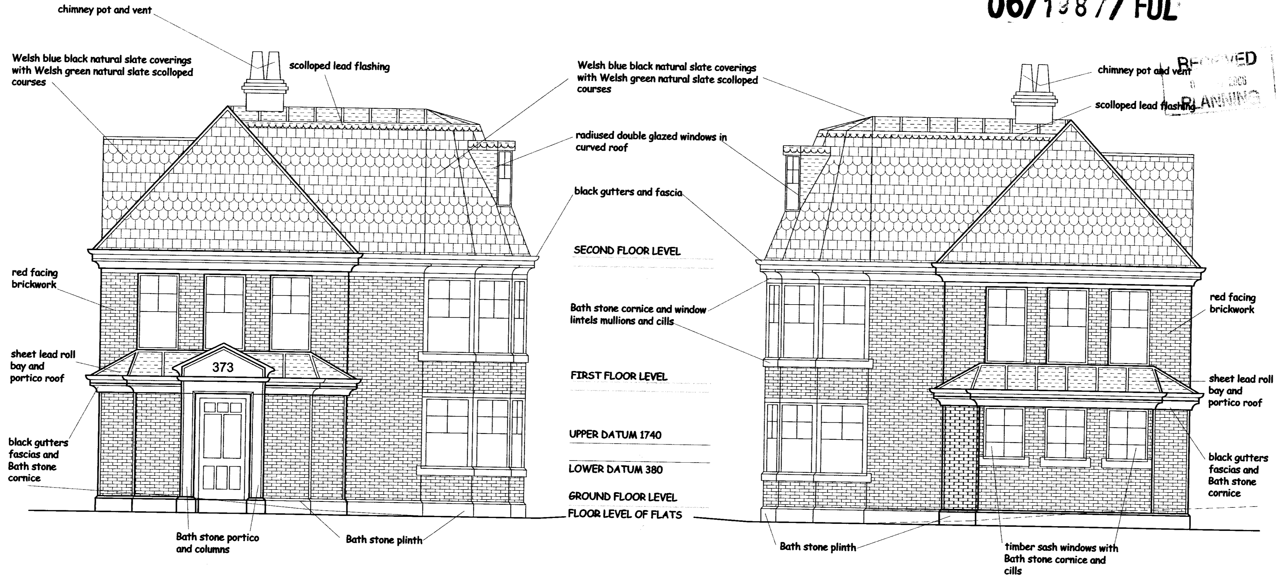
ELEVATION TO HIGH PARK ROAD
