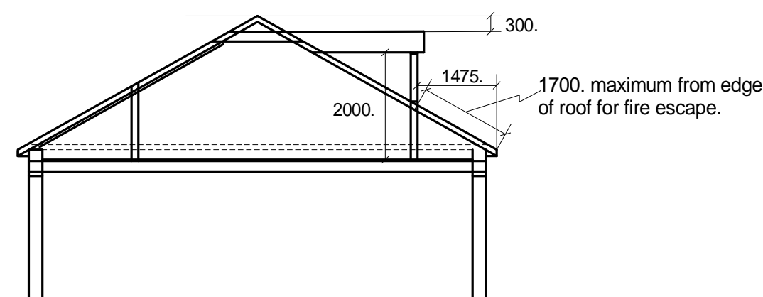
SECTION X-X scale 1:100
