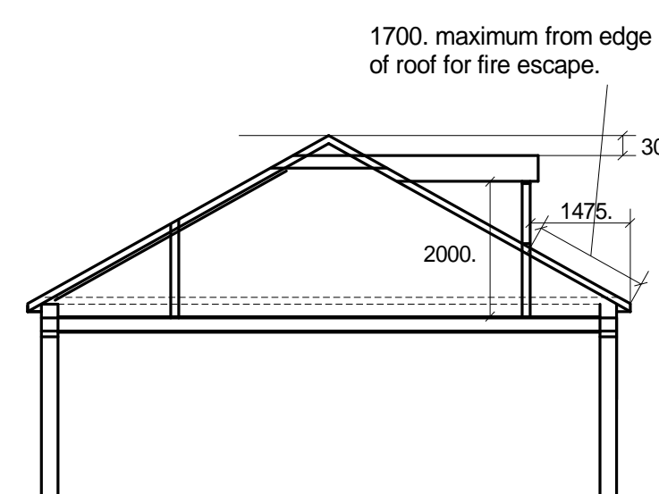
SECTION X-X scale 1:100
