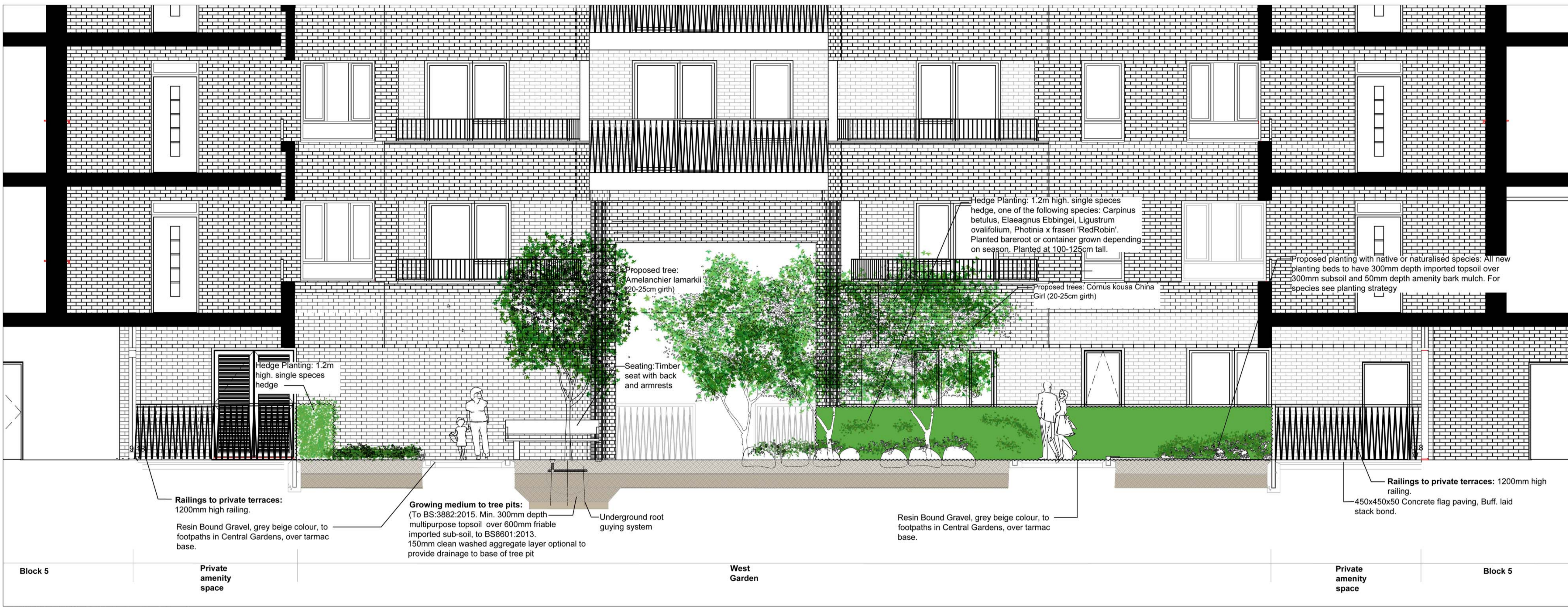
SECTIONAL ELEVATION C-C - West Garden
