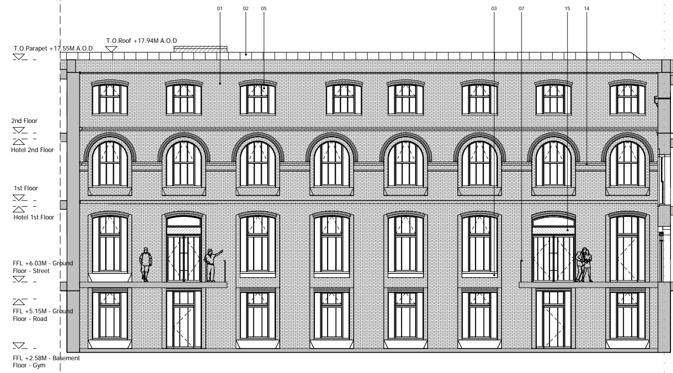
3 PROPOSED NORTH 3 1 : 100
