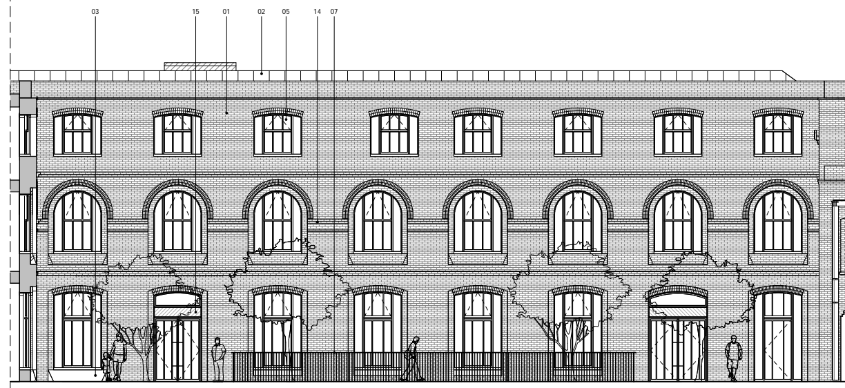
1 PROPOSED NORTH 2 1 : 100
