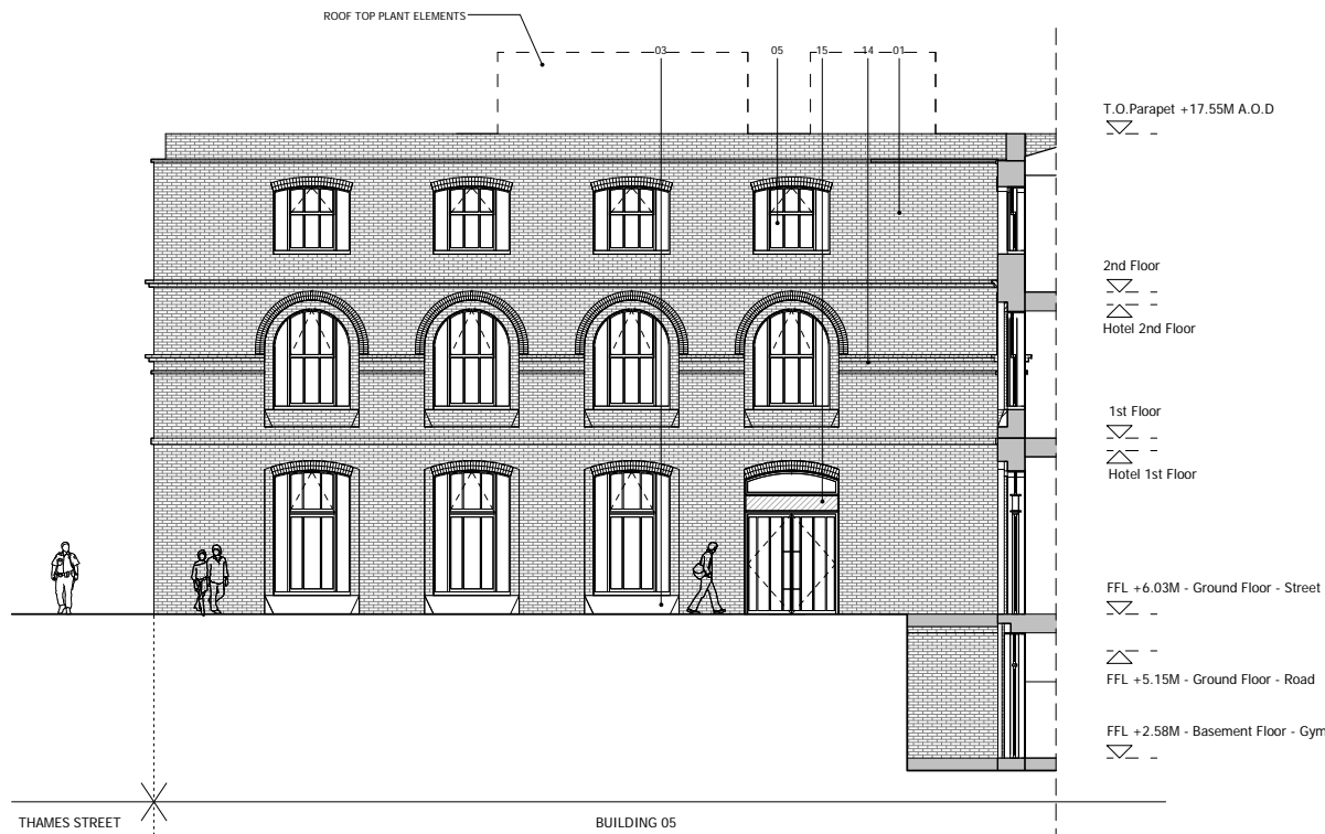
2 PROPOSED WEST ELEVATION 1 1 : 100
