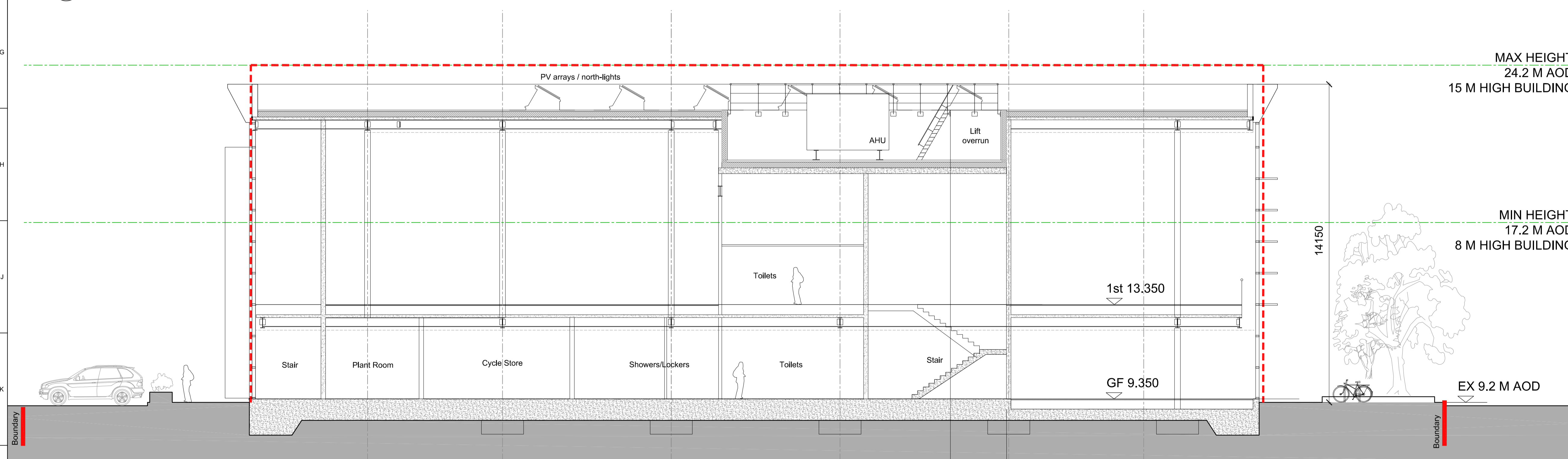
2 SECTION B-B SCALE 1:100
