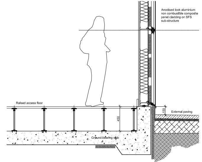
D rainscreen cladding full height 1:50
