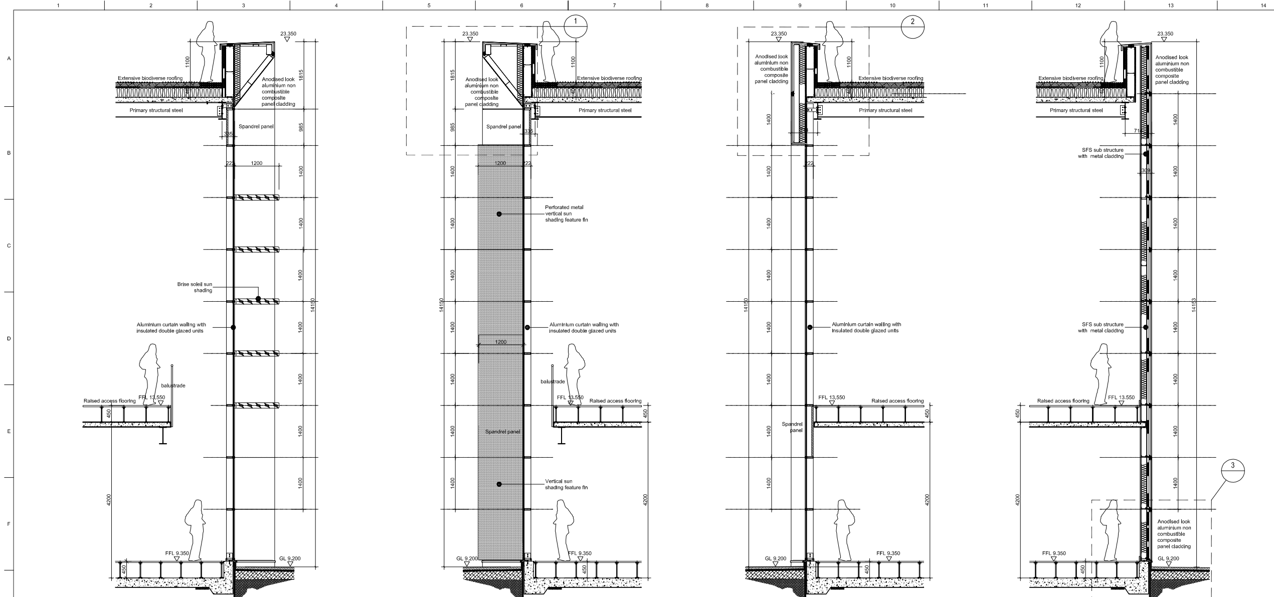
A curtain walling/brise soleil 1:50
