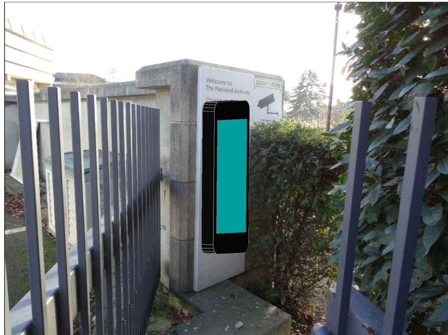
POSITION A. Screen to be pillar mounted 450mm above ground
