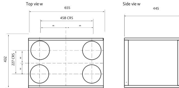
Figure 10. MRXBOX-SIL3.
