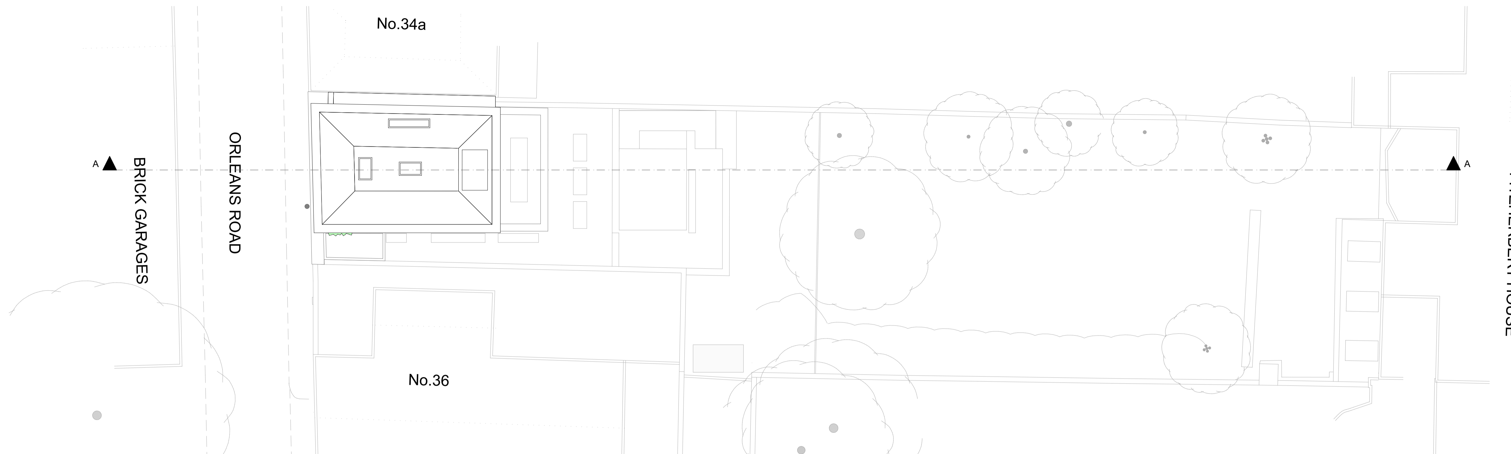
Roof Plan 1:100 @ A1
