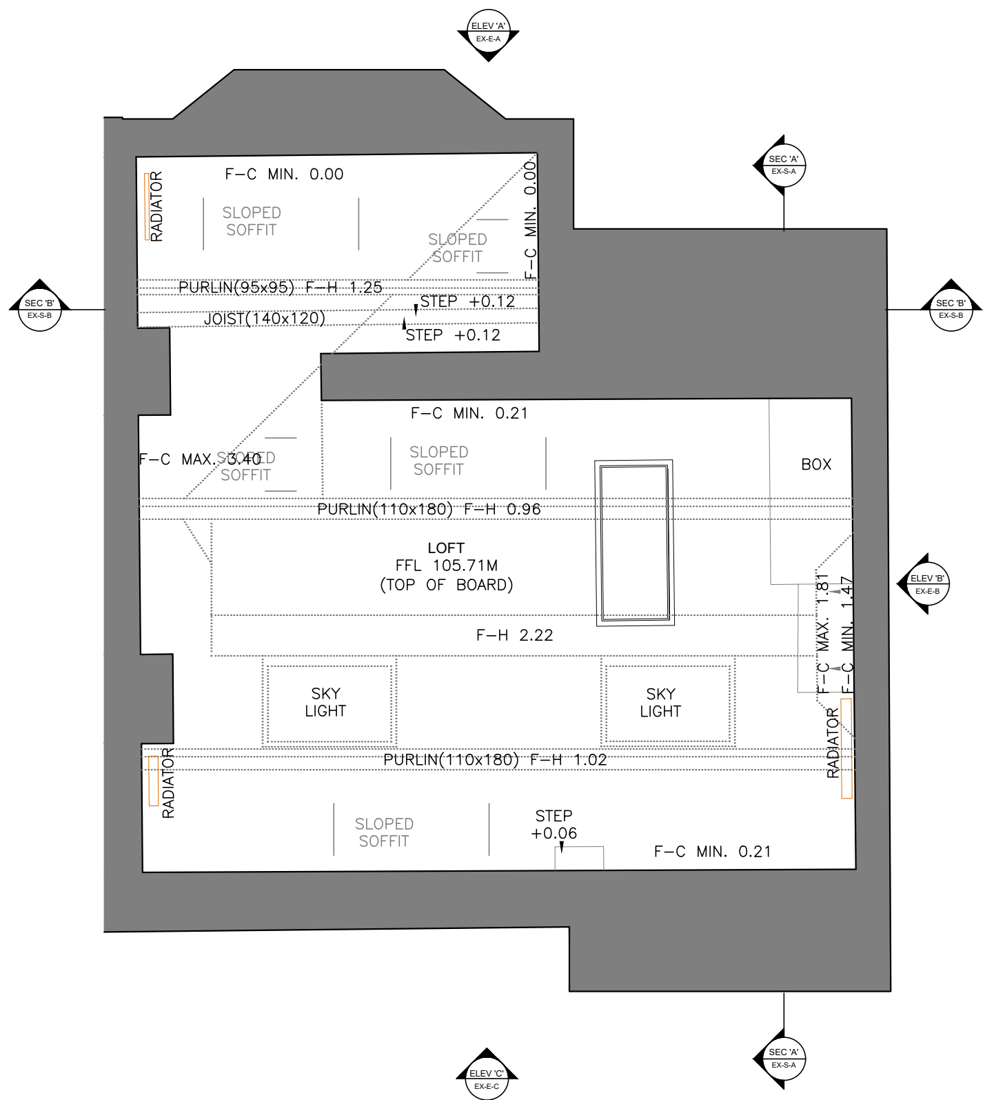
1 | SECOND FLOOR PLAN AS PRE-EXISTING EX-P-102 | SCALE: 1:50 @ A3 // 1:25 @ A1
