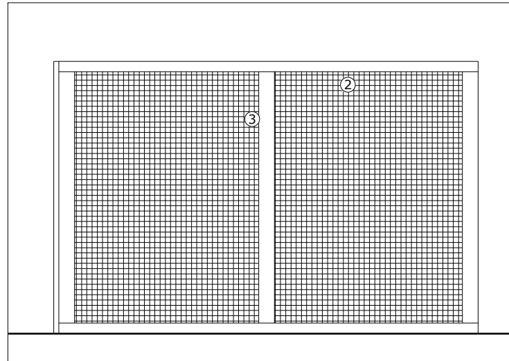
South Elevation
