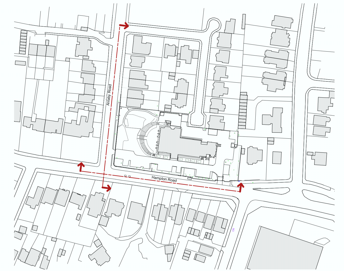
1 Key to Sections Scale: 1:1500
