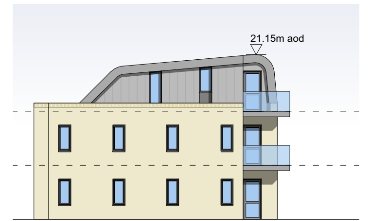
WEST ELEVATION (1:100)
