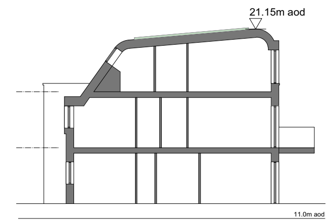
SECTION AA (1:100)
