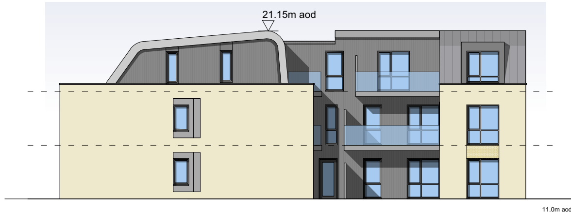
NORTH ELEVATION (1:100)
