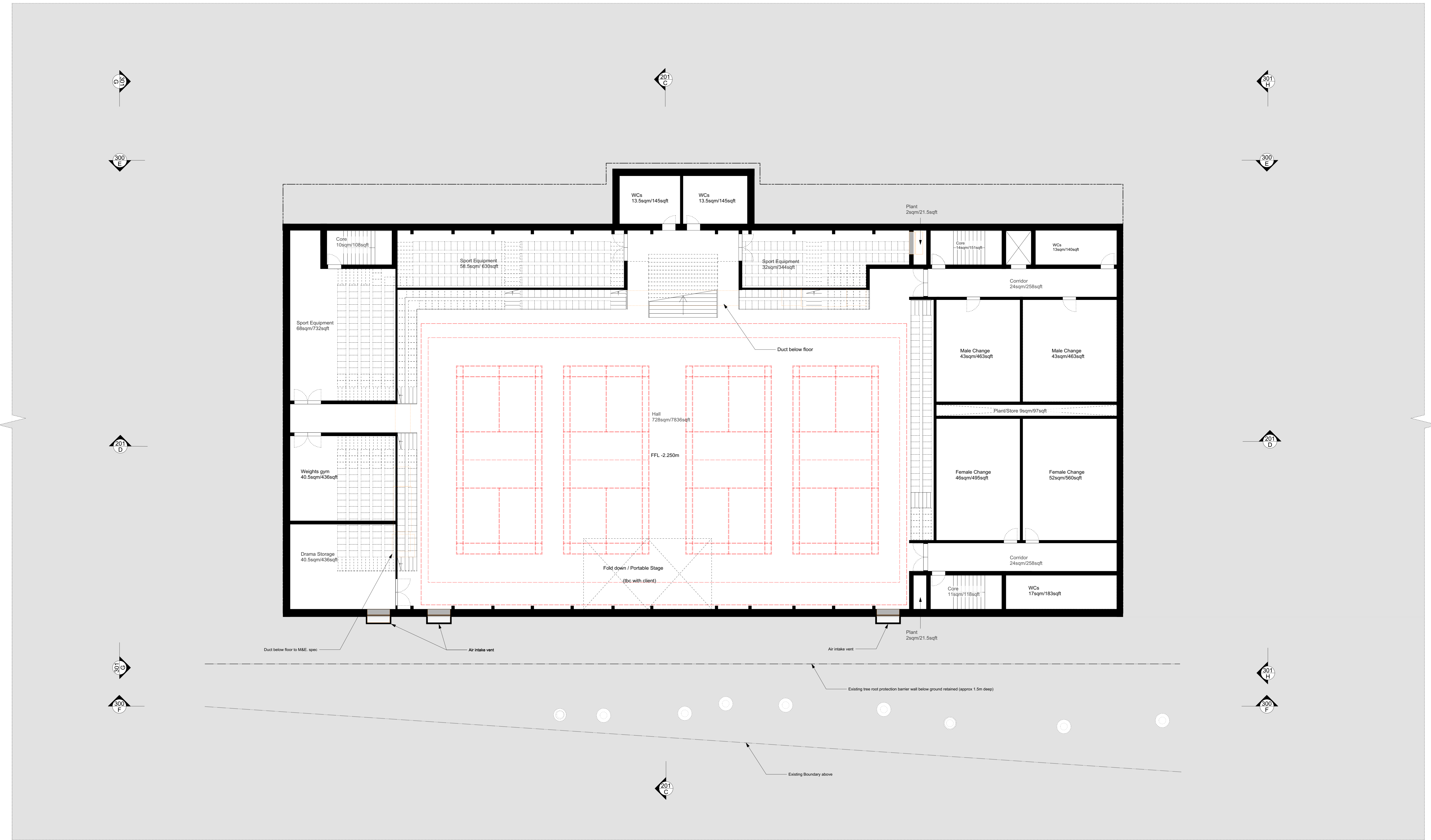
Proposed Basement Plan 1:100@A0
