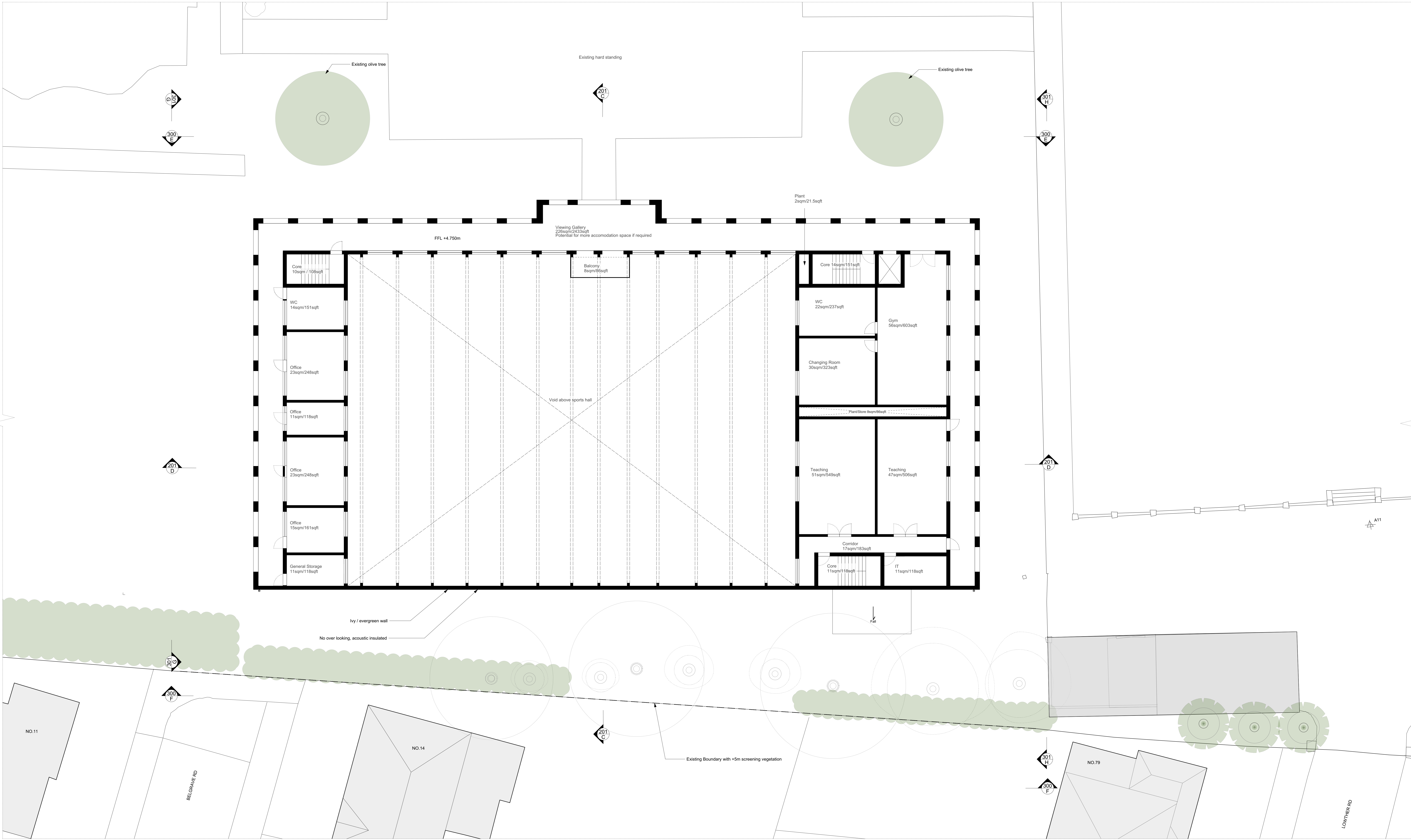
Proposed First Floor Plan 1:100@A0
