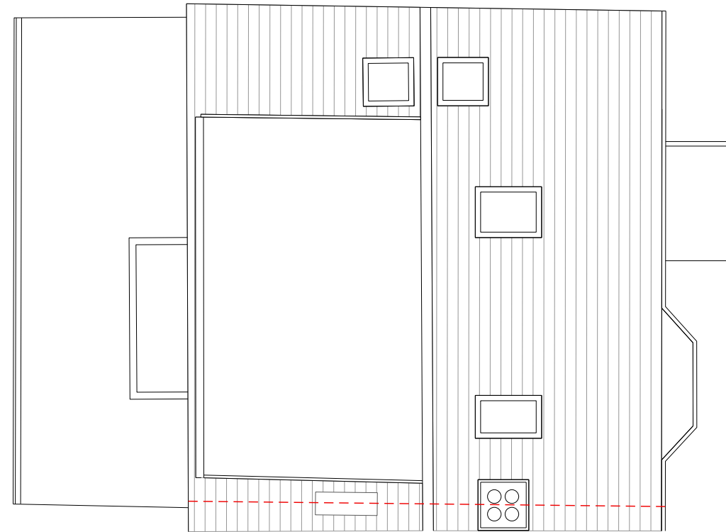
ROOF PLAN
