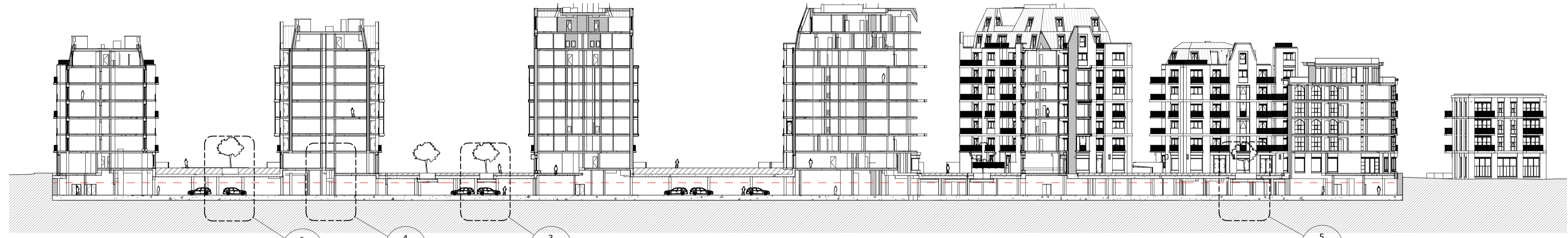
1 Basement Section_Phase 01_002 1 : 500
