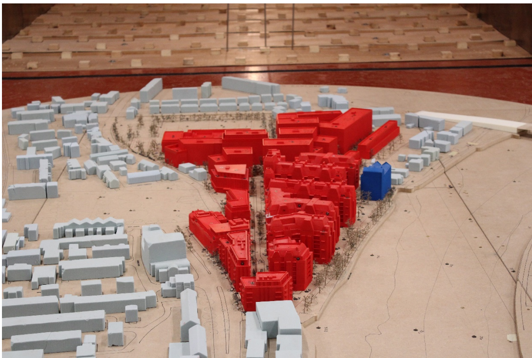
Figure 14 - Proposed Development with Landscaping and Existing Surrounding Buildings (Configuration 2) - View in the Wind Tunnel (from the East)
