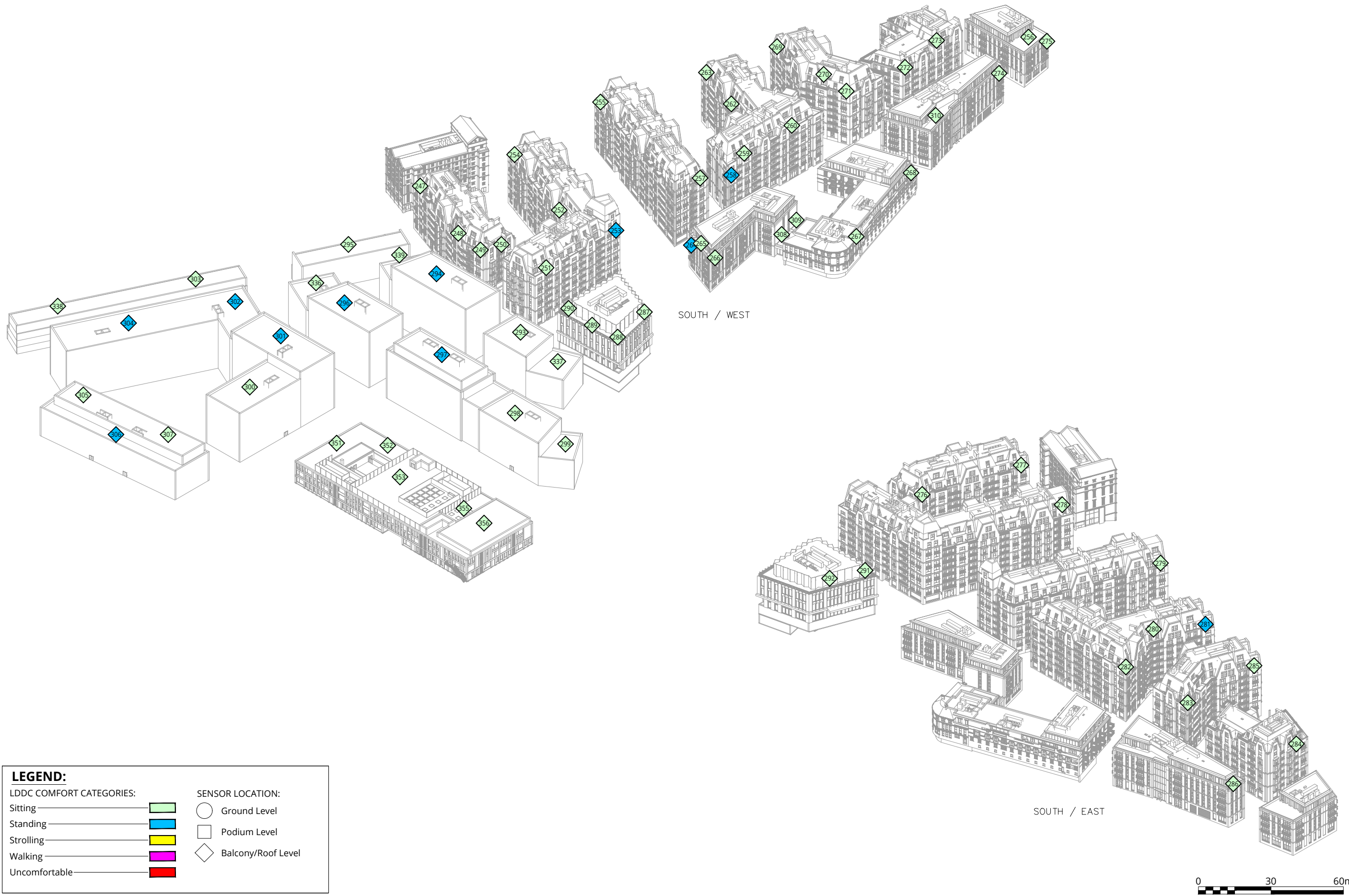
Pedestrian Wind Comfort Conditions - Isometric Views Configuration 2: Proposed Development with Landscaping and the Existing Surrounding Buildings Summer Season
