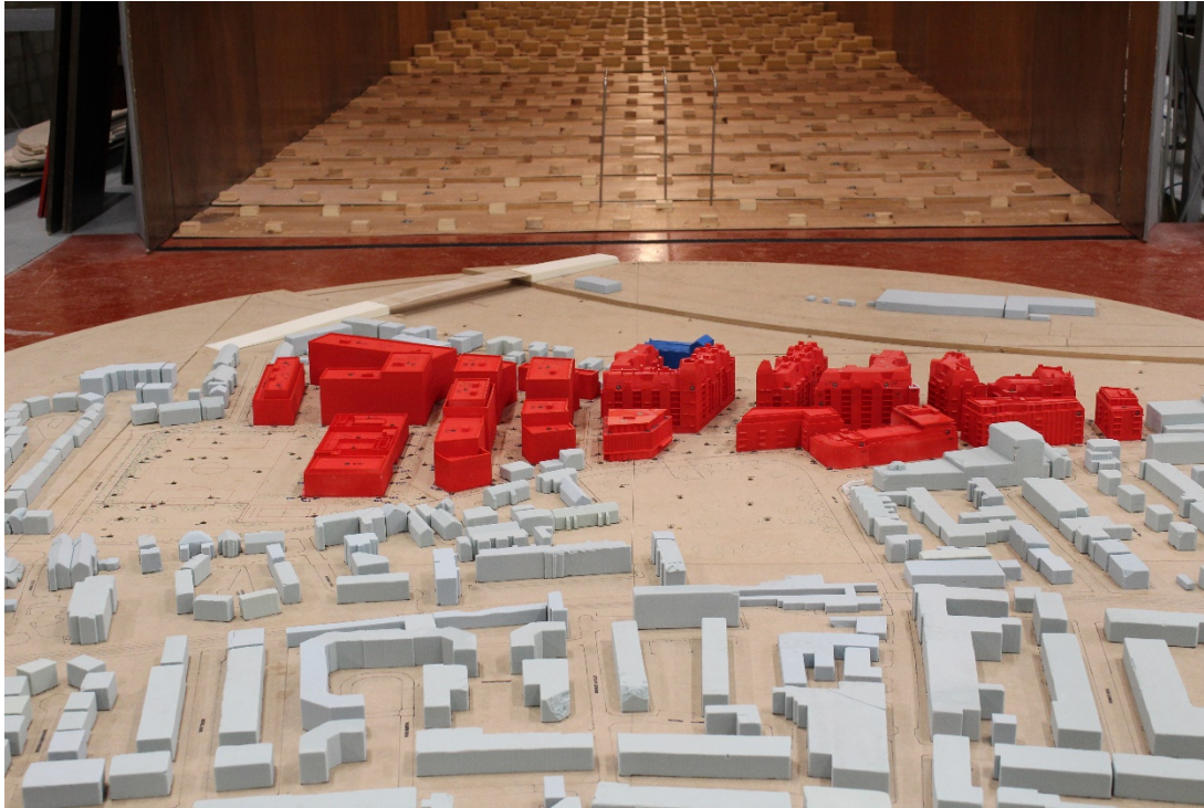
Figure 11 - Proposed Development and Existing Surrounding Buildings (Configuration 1) - View in the Wind Tunnel (from the South)
