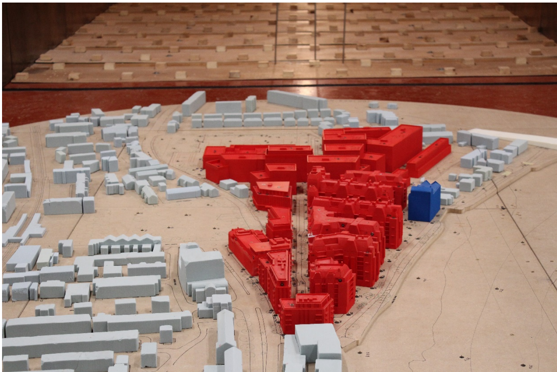
Figure 12 - Proposed Development and Existing Surrounding Buildings (Configuration 1) - View in the Wind Tunnel (from the East)
