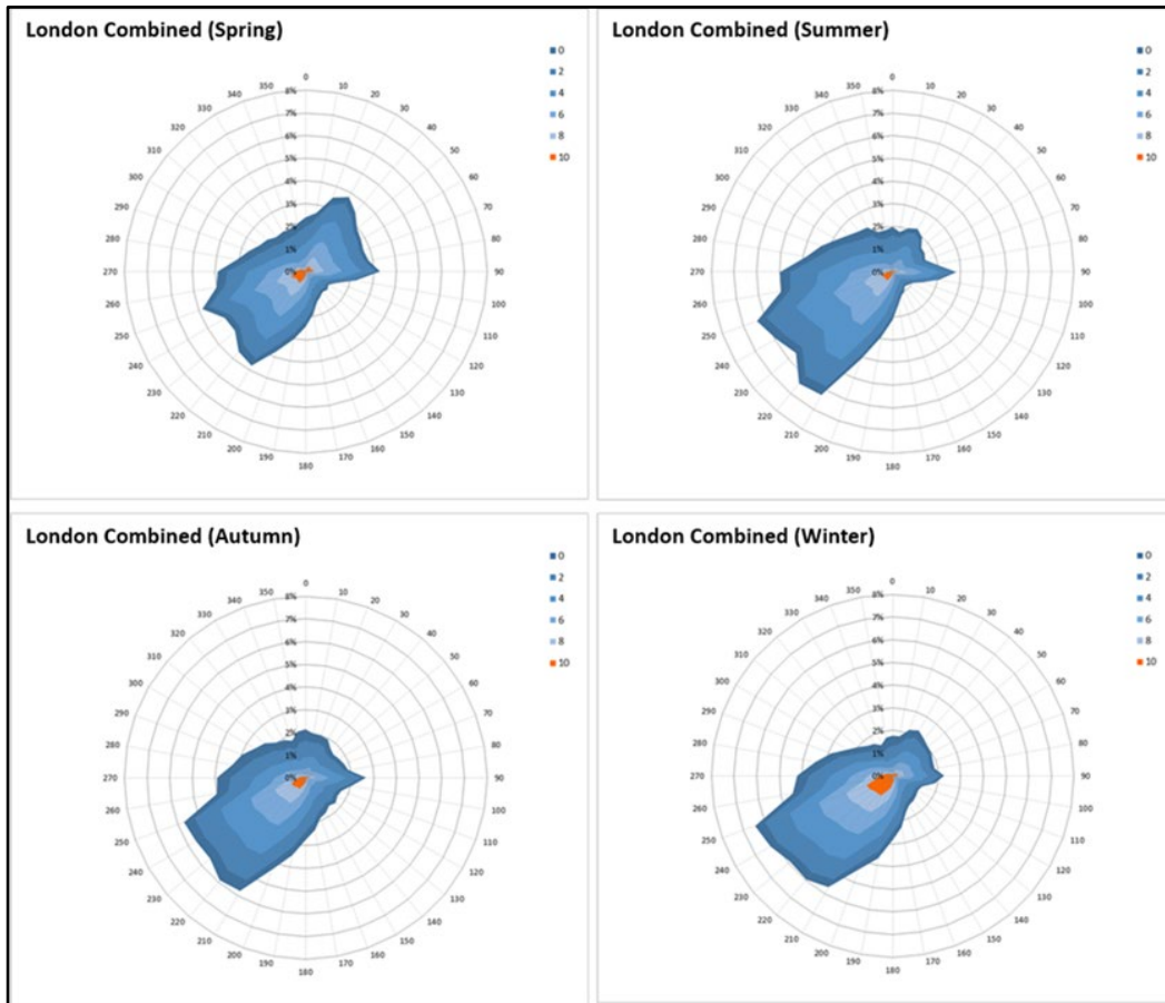
Figure 15: Seasonal wind roses from London Combined (in m/s) - (Radial axis indicates the percentage of time for which the stated threshold is exceeded)
