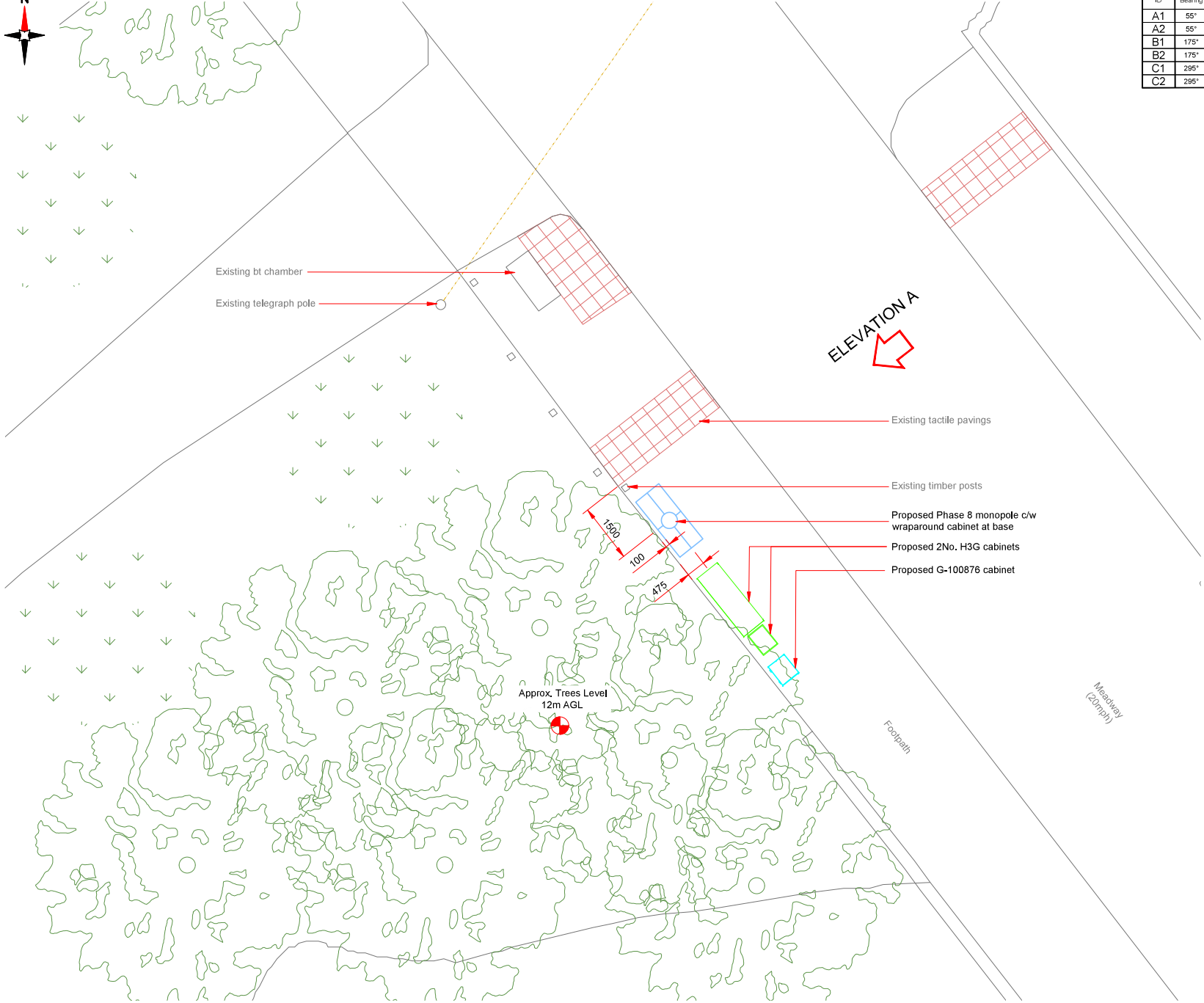
PROPOSED H3G SITE PLAN 0 1:100 2m 4
