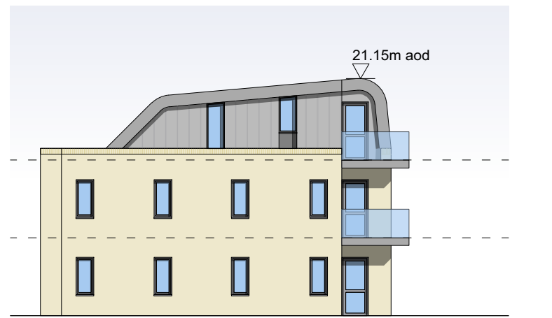
WEST ELEVATION (1:100)
