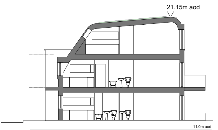
SECTION AA (1:100)
