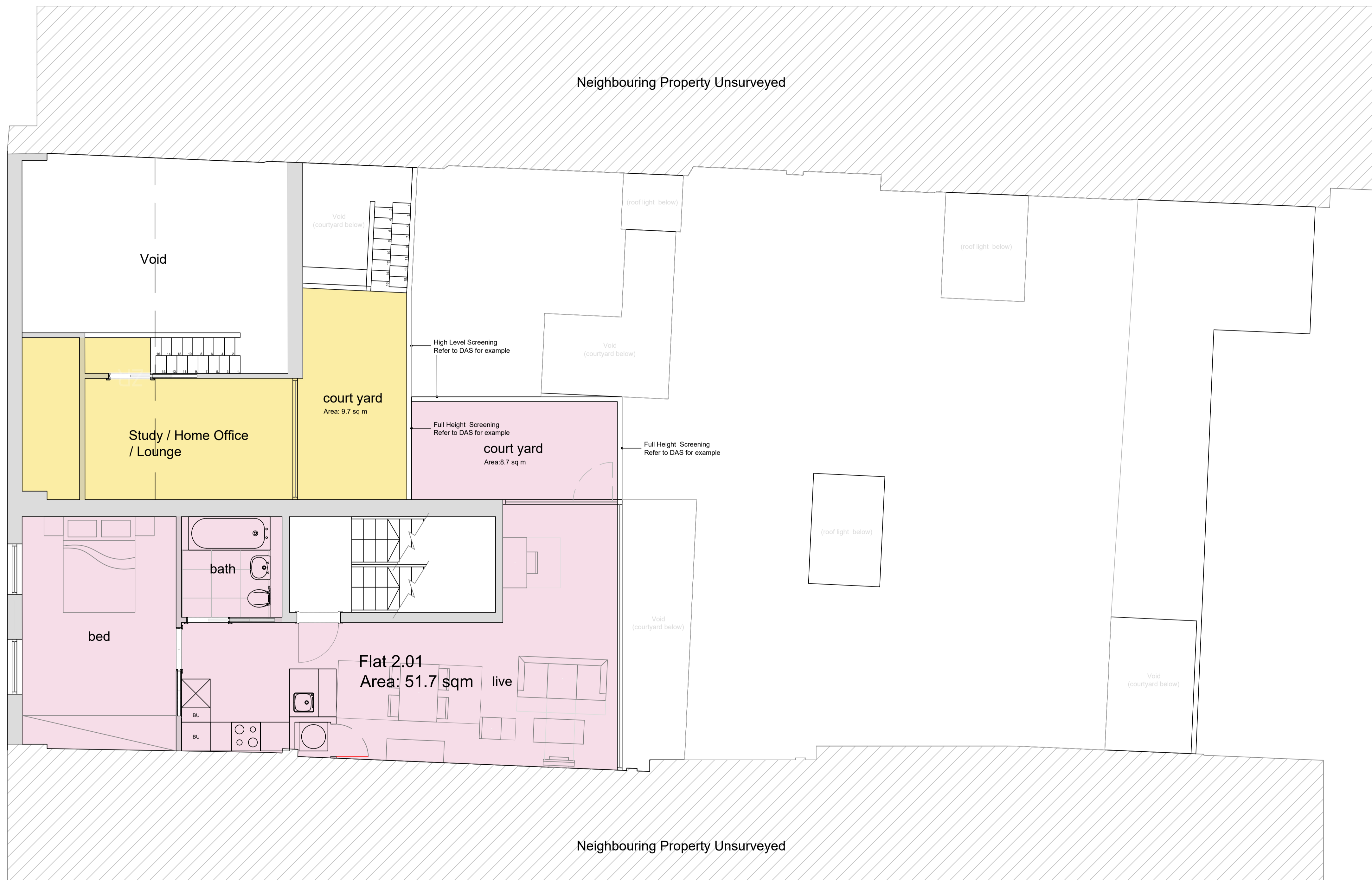
Second Floor Plan Scale: 1/50
