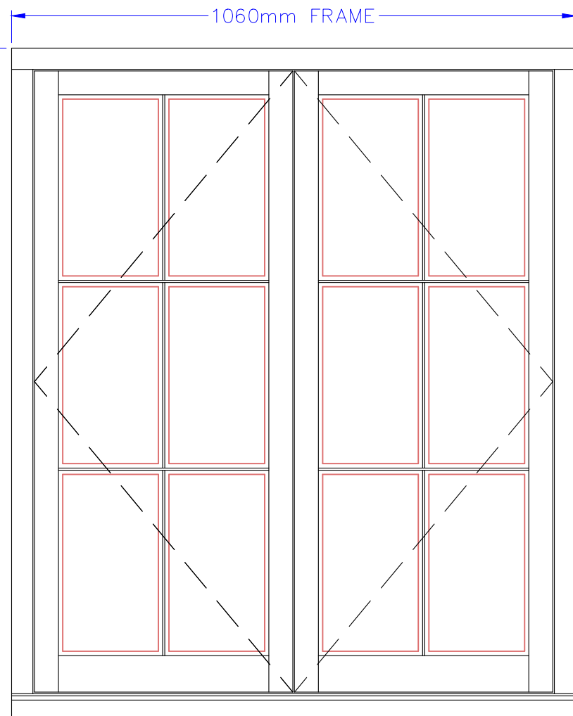
FRONT ELEVATION
