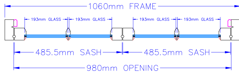
PLAN SECTION
