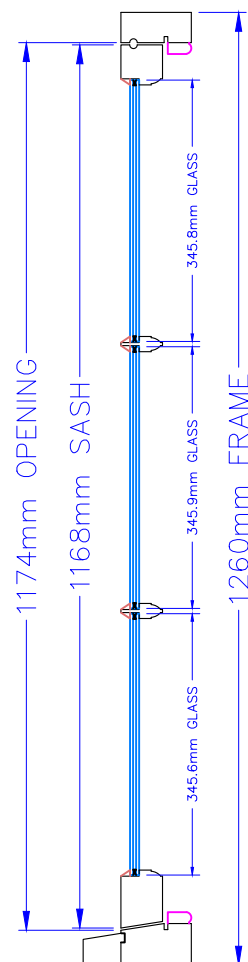
SECTION
