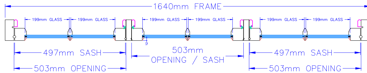
PLAN SECTION
