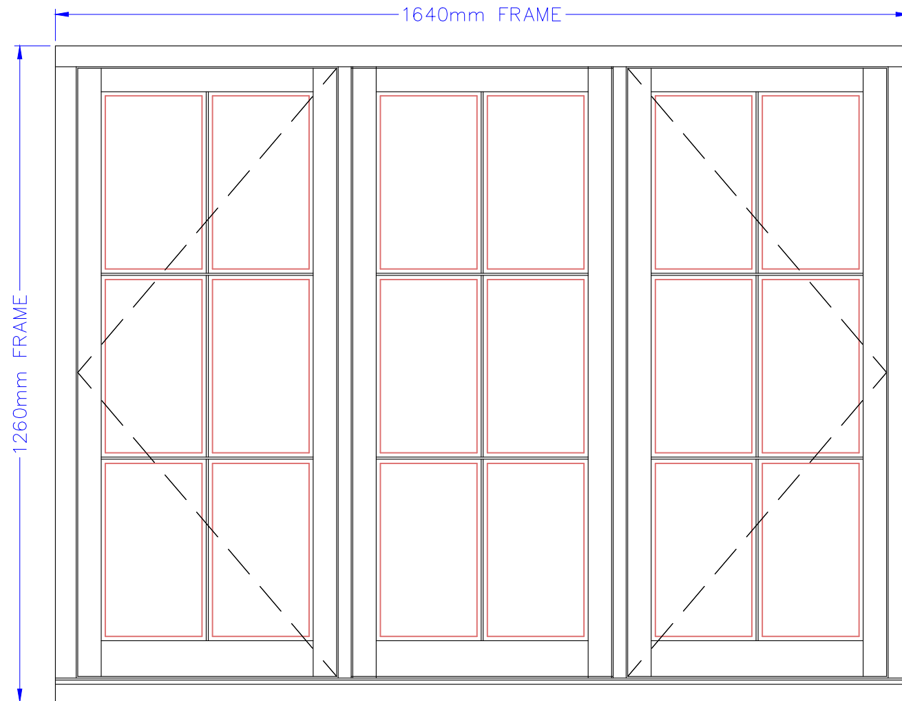
FRONT ELEVATION
