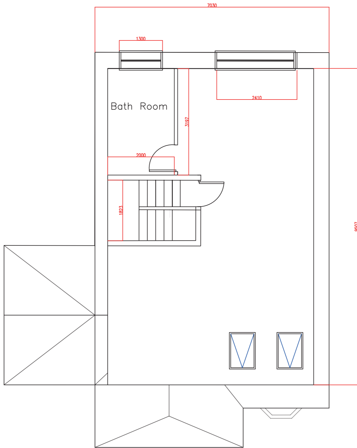
PROPOSE LOFT FLOOR PLAN
