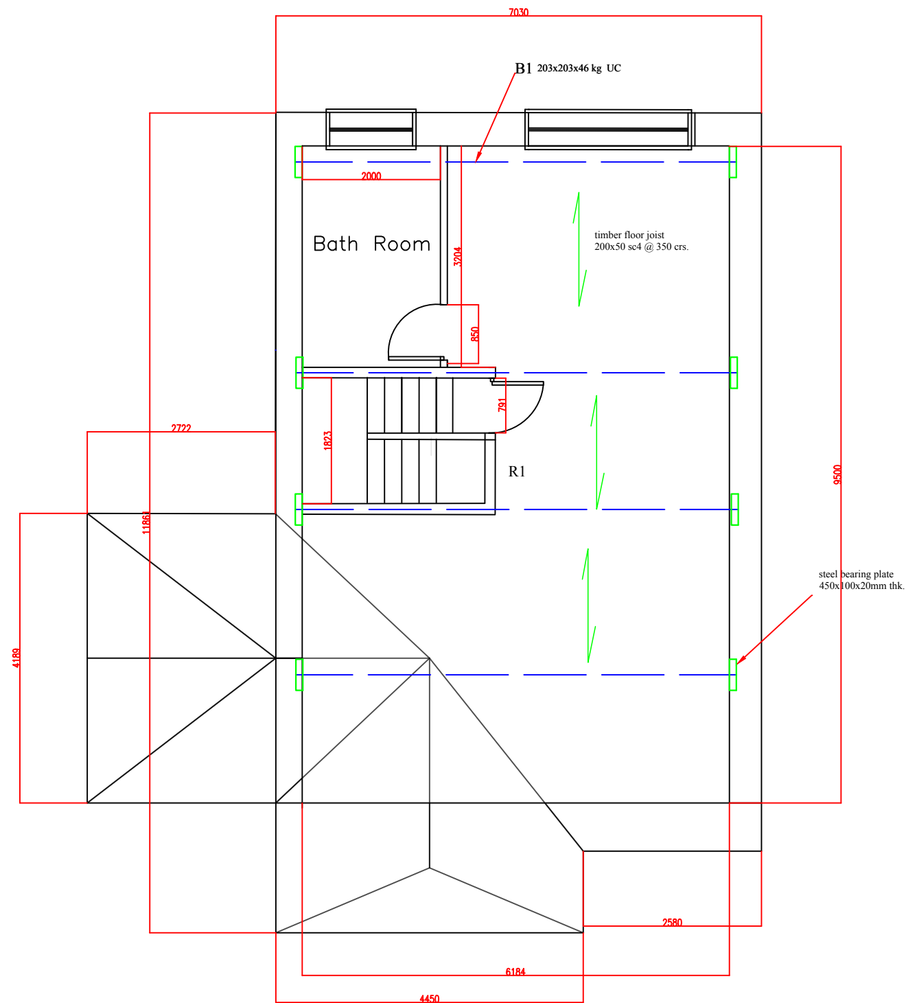
PROPOSE LOFT FLOOR PLAN HIP VALLEY DETAIL
