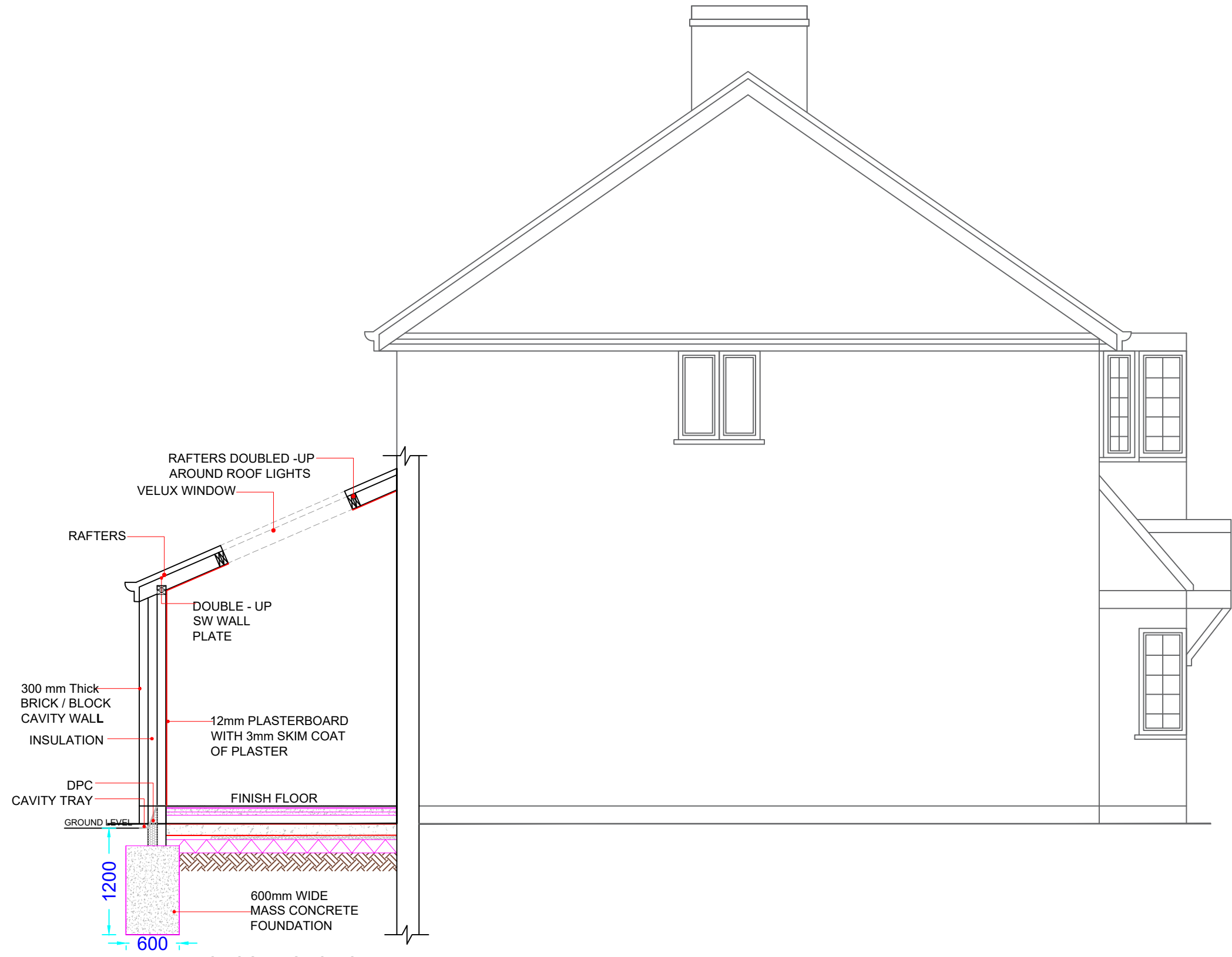
PROPOSED SECTION AA SCALE 1:50
