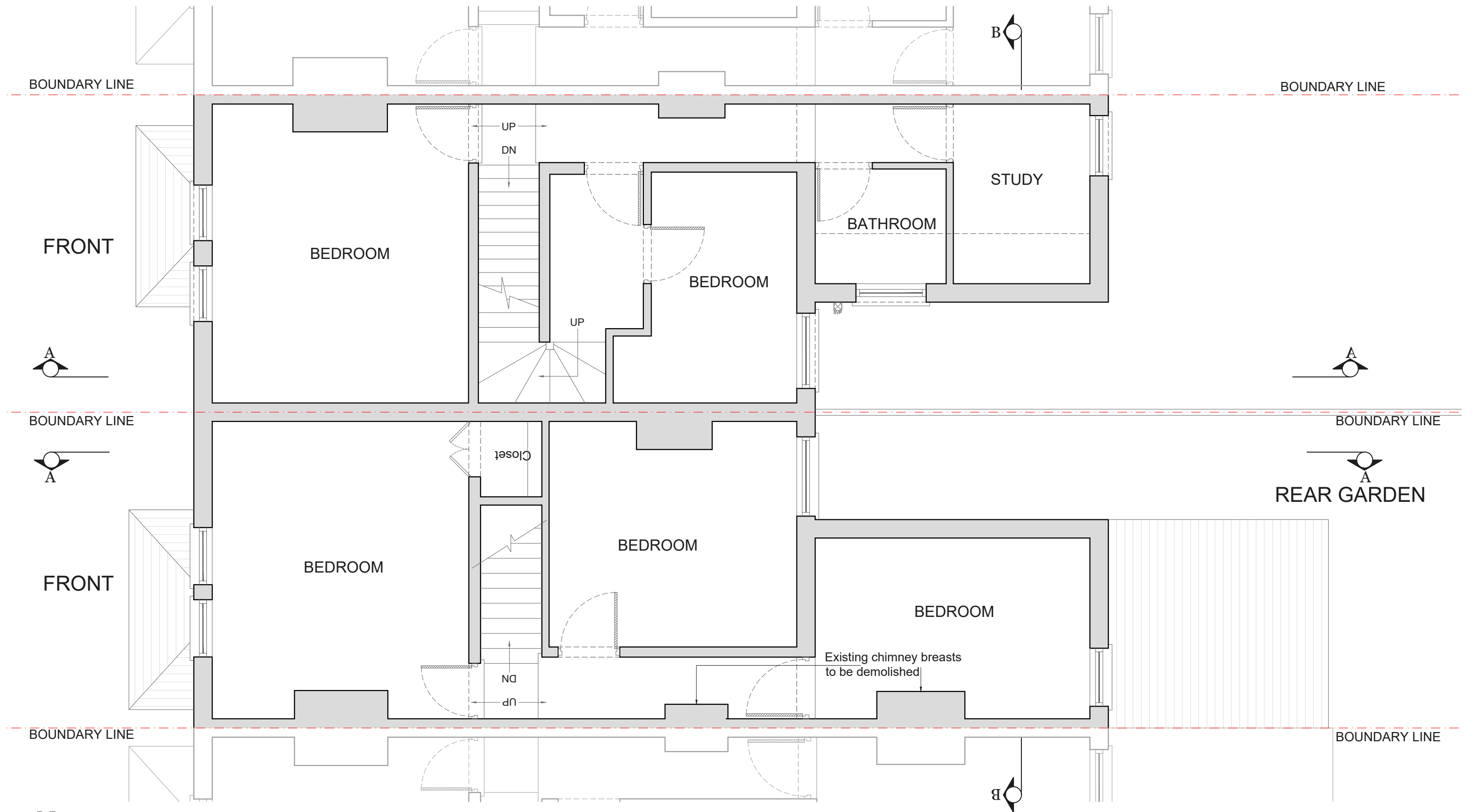
EXISTING FIRST FLOOR PLANS (No. 05 AND No. 03) SCALE 1:50
