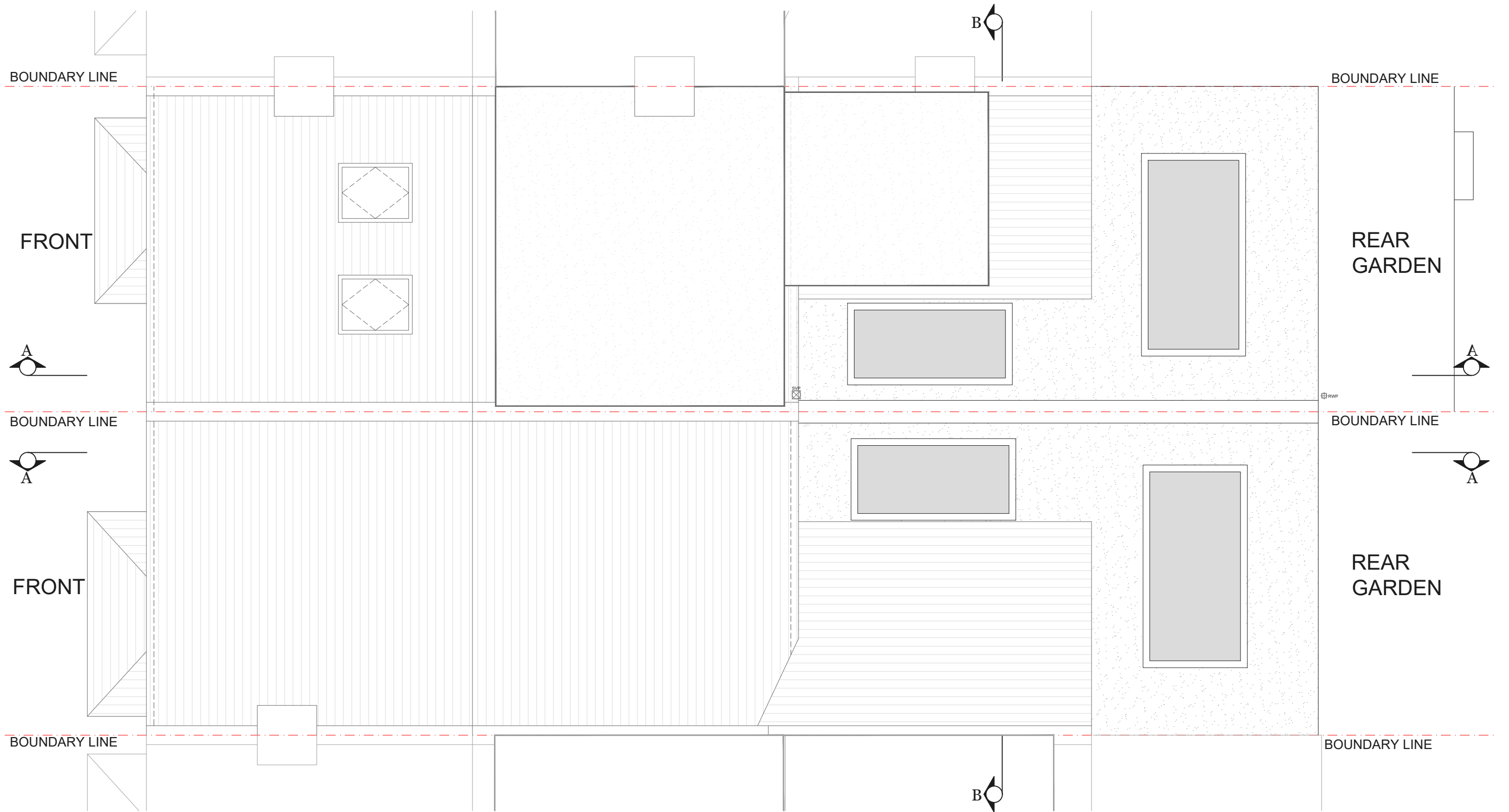
PROPOSED ROOF TOP PLANS (No. 05 AND No. 03) SCALE 1:50
