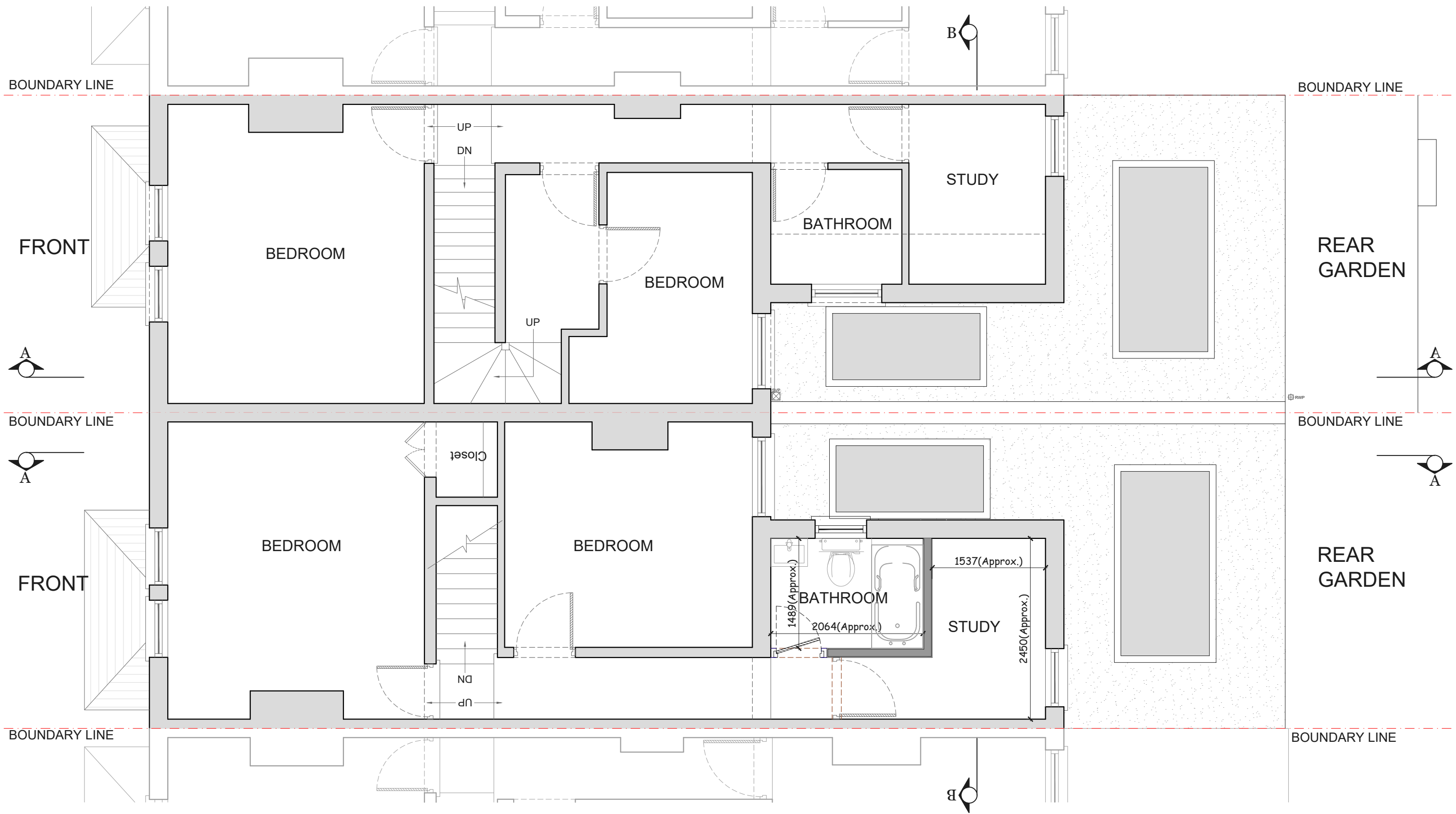
PROPOSED FIRST FLOOR PLANS (No. 05 AND No. 03) SCALE 1:50
