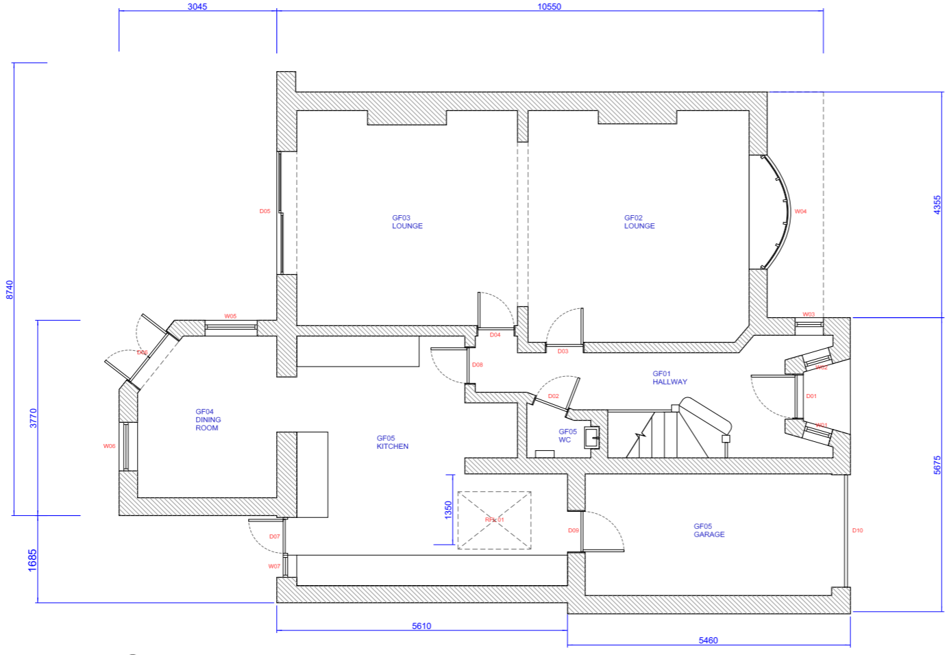
P1 EXISTING GROUND FLOOR 1:100
