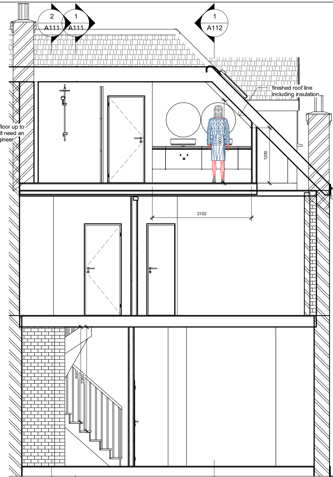
2 PROPOSED SECTION 5 1 : 50
