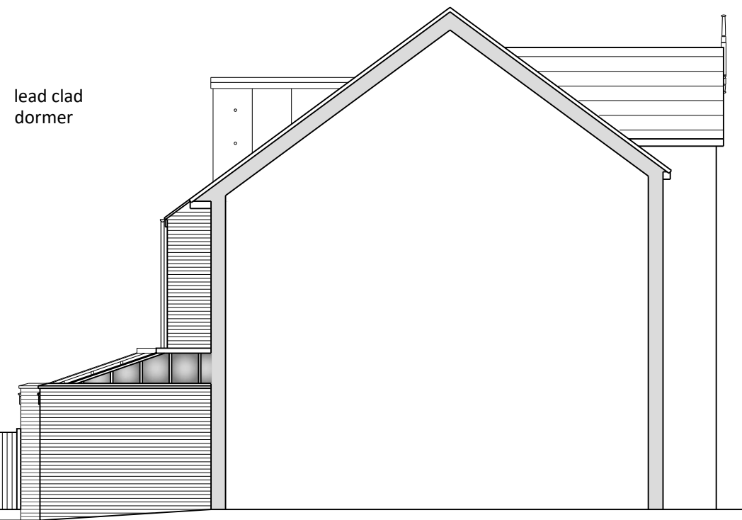
E1 Side Section/Elevation Proposed 1:100 @ A3
