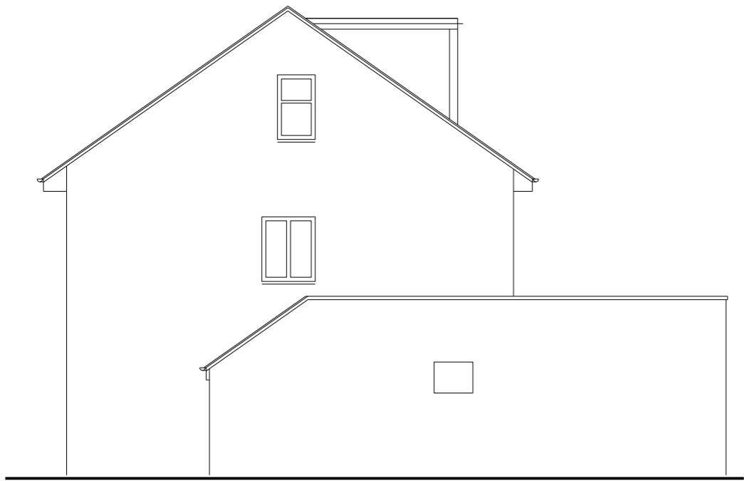
SIDE ELEVATION facing No.2
